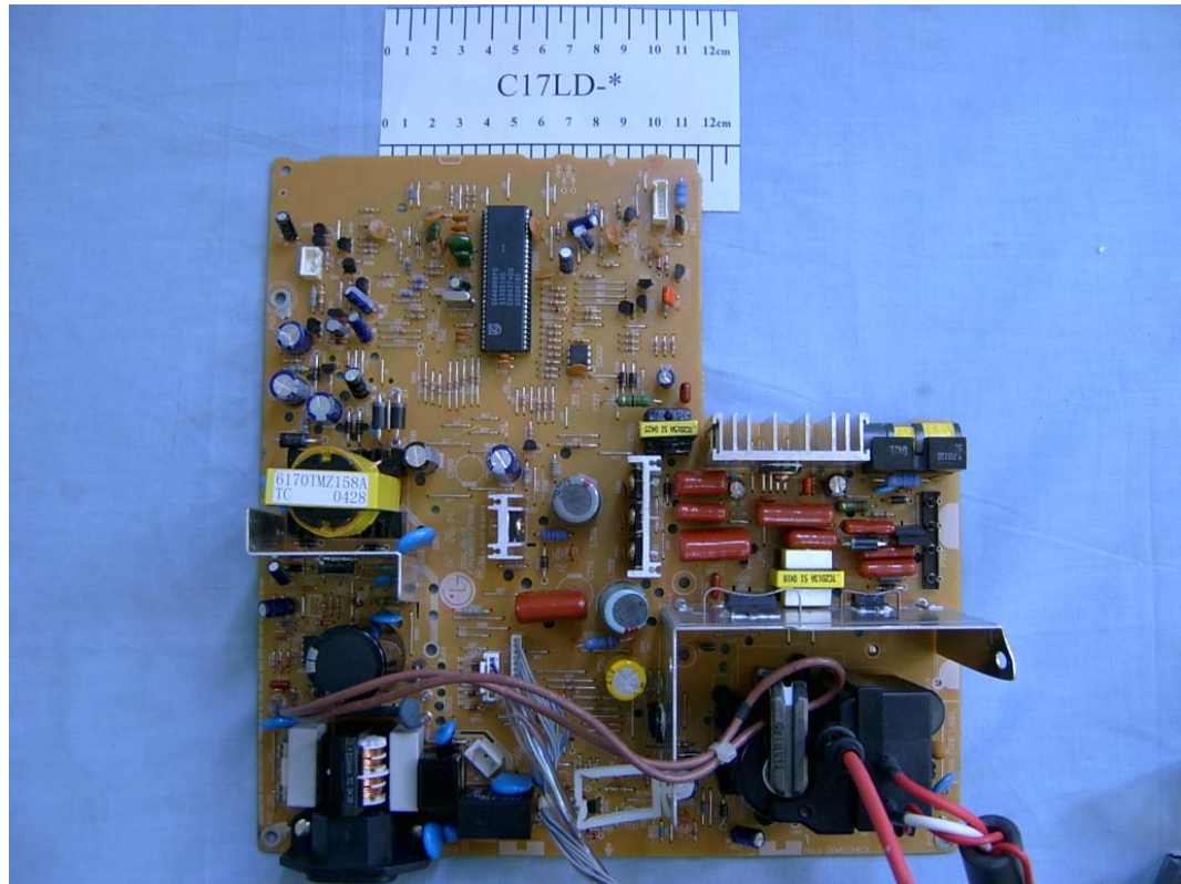
FIGURE 5 COLOR MONITOR (M/N: C17LD-*) MAIN BOARD (COMPONENT SIDE)
