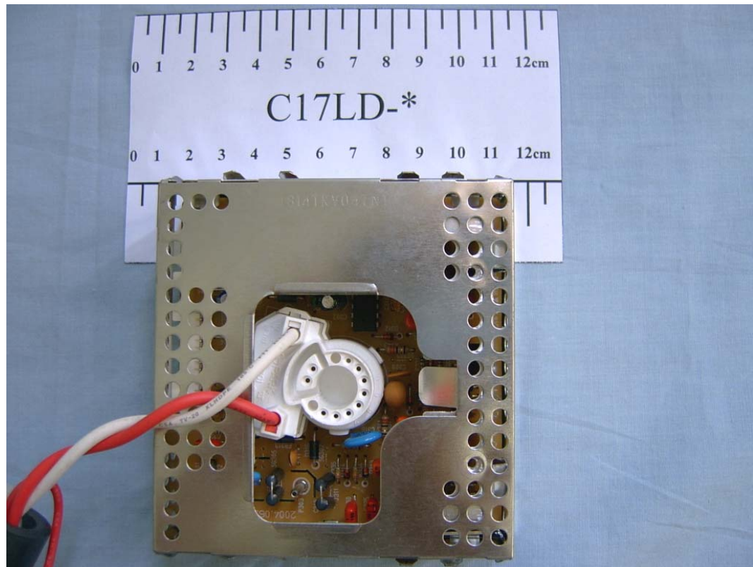
FIGURE 7 COLOR MONITOR (M/N: C17LD-*) CRT BOARD WITH SHIELDED (COMPONENT SIDE)
