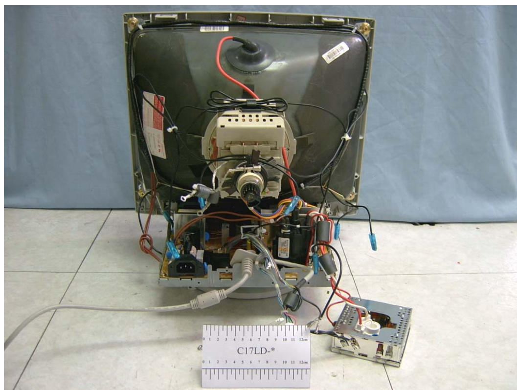
FIGURE 2 COLOR MONITOR (M/N: C17LD-*) COVER REMOVED 2
