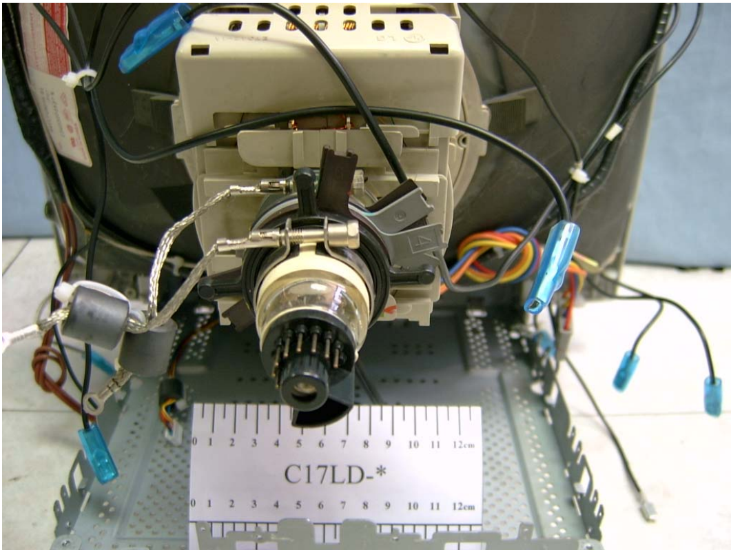
FIGURE 3 COLOR MONITOR (M/N: C17LD-*) CRT TUBE
