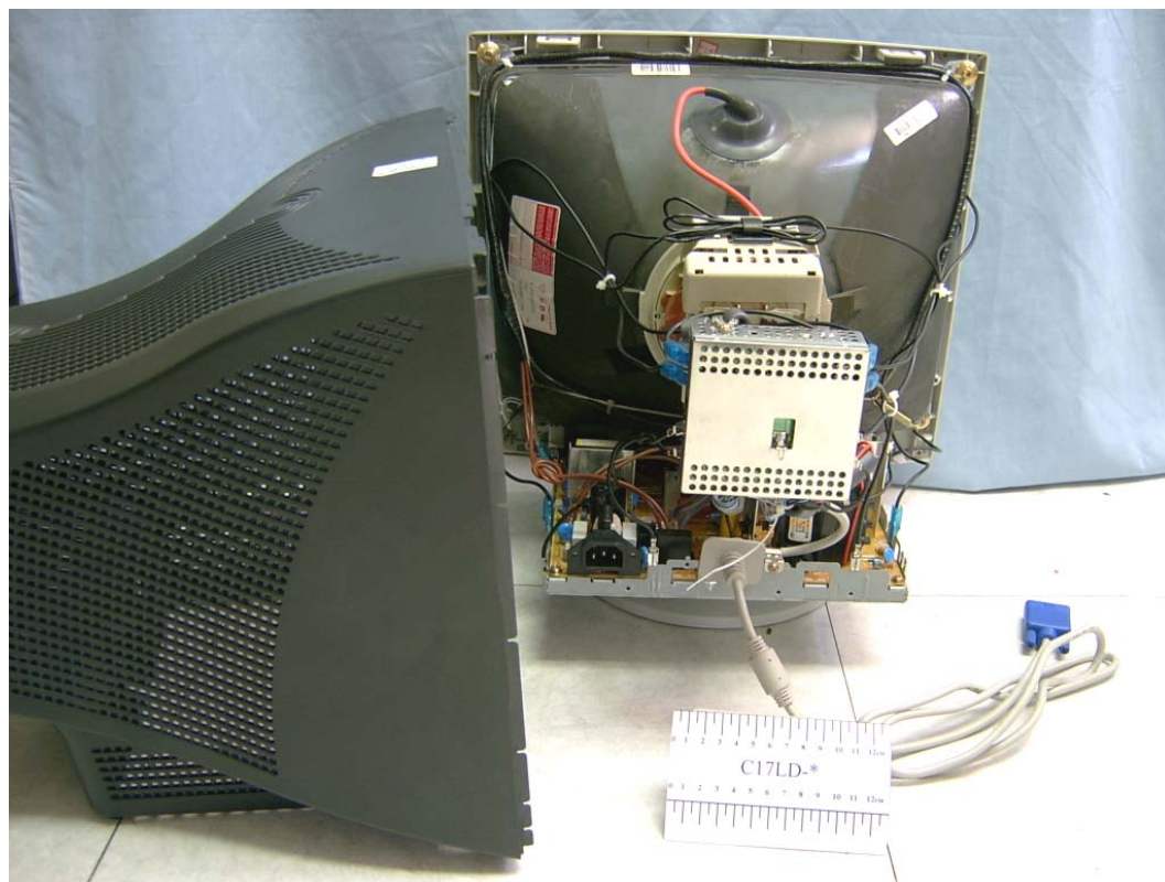
FIGURE 1 COLOR MONITOR (M/N: C17LD-*) COVER REMOVED 1
