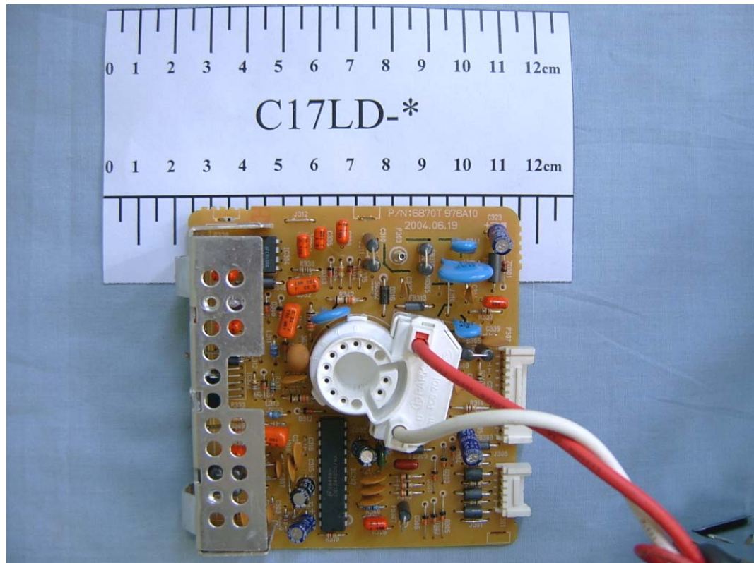
FIGURE 9 COLOR MONITOR (M/N: C17LD-*) CRT BOARD (COMPONENT SIDE)
