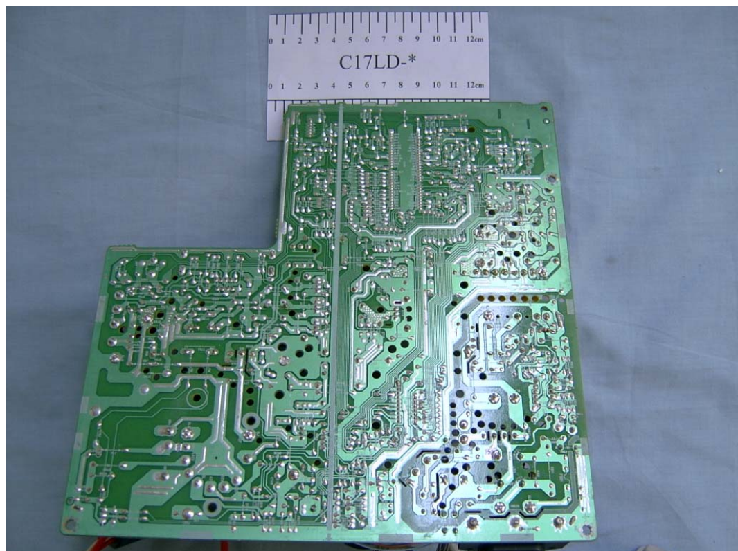
FIGURE 6 COLOR MONITOR (M/N: C17LD-*) MAIN BOARD (SOLDERED SIDE)
