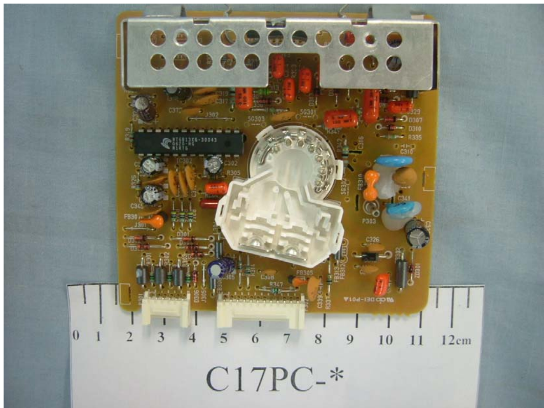
FIGURE 17 CRT MONITOR (M/N: C17PC-*) MAIN BOARD 2 (COMPONENT SIDE)
