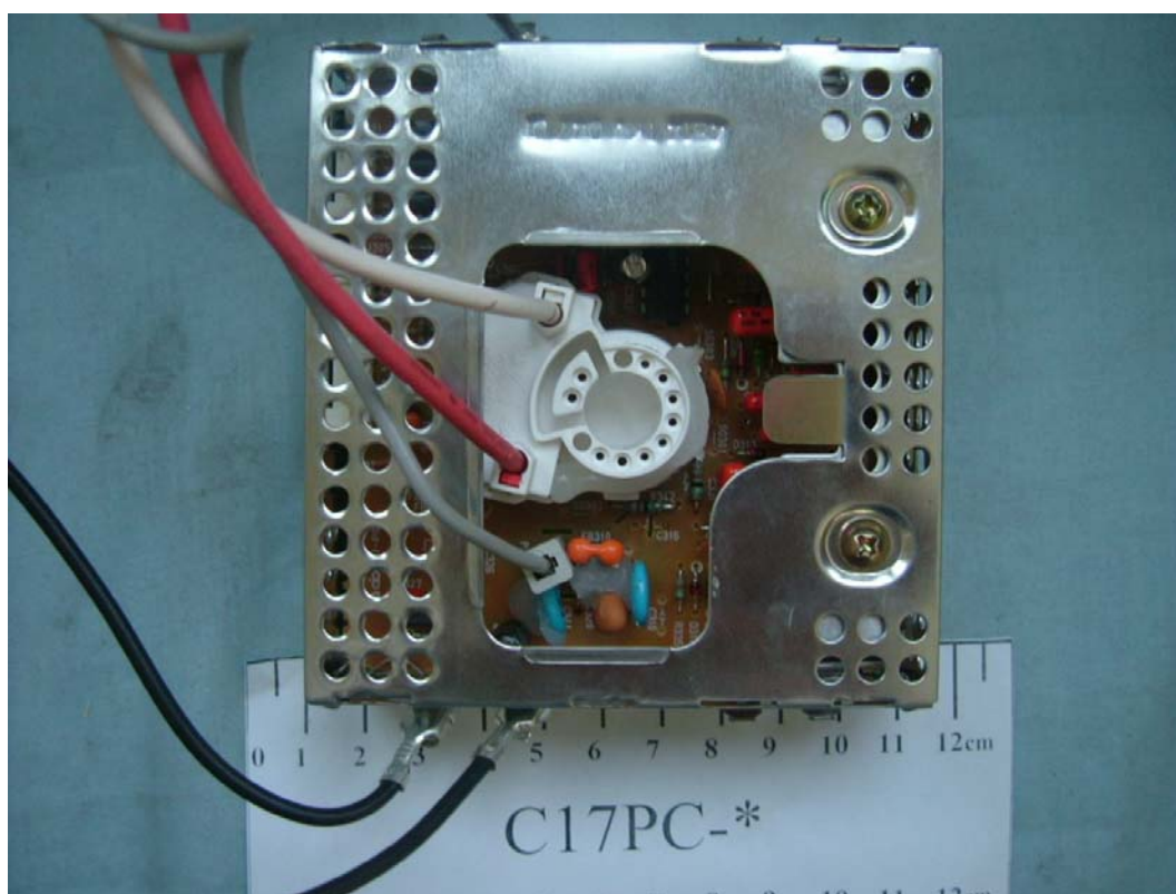
FIGURE 15 CRT MONITOR (M/N: C17PC-*) MAIN BOARD 2
