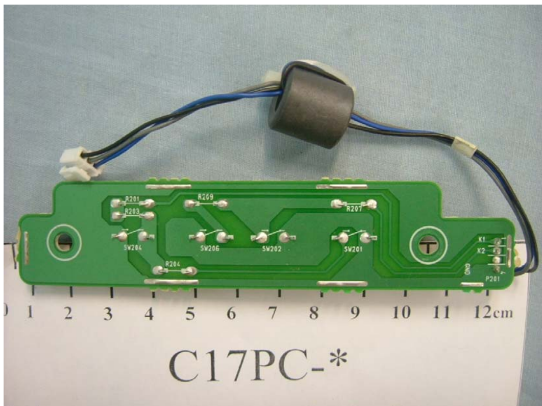
FIGURE 14 CRT MONITOR (M/N: C17PC-*) BUTTON CONTROL BOARD (SOLDERED SIDE)
