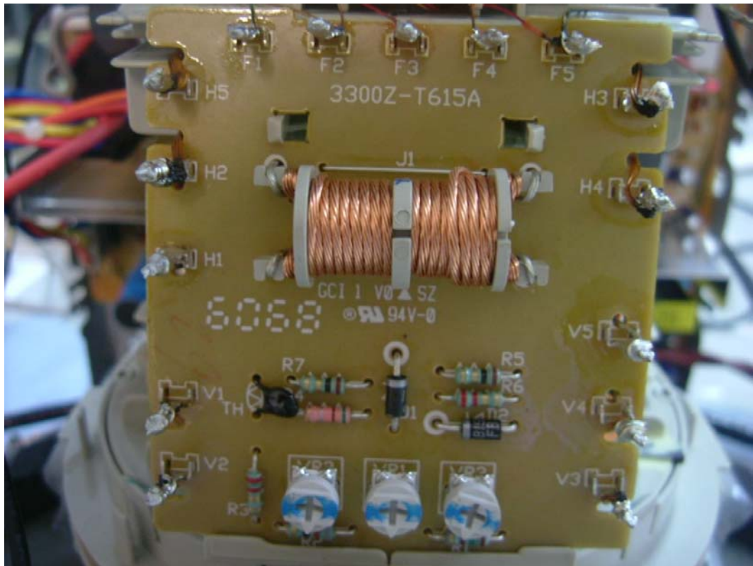
FIGURE 21 CRT MONITOR (M/N: C17PC-*) MAIN BOARD 3 (COMPONENT SIDE)
