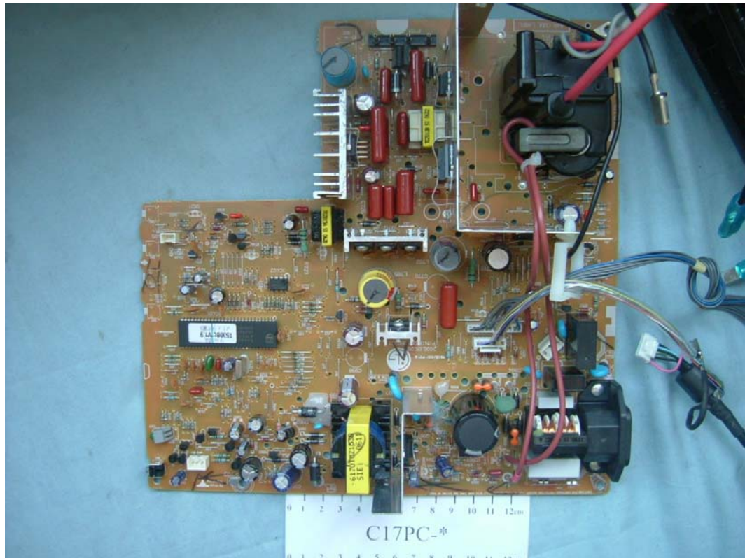
FIGURE 11 CRT MONITOR (M/N: C17PC-*) MAIN BOARD 1 (COMPONENT SIDE)
