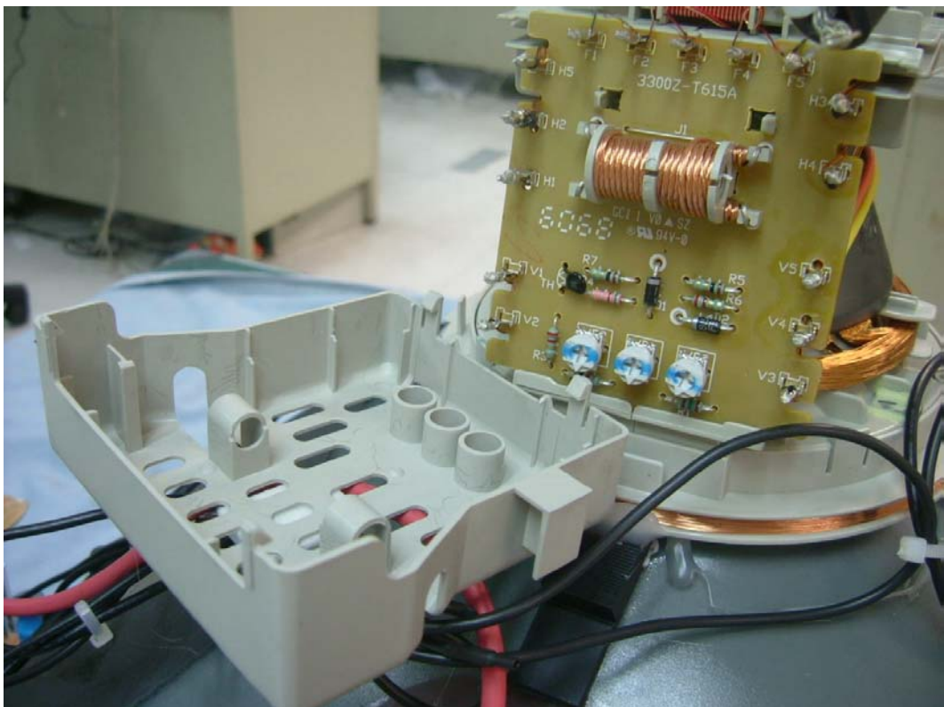
FIGURE 20 CRT MONITOR (M/N: C17PC-*) MAIN BOARD 3 COVER REMOVED
