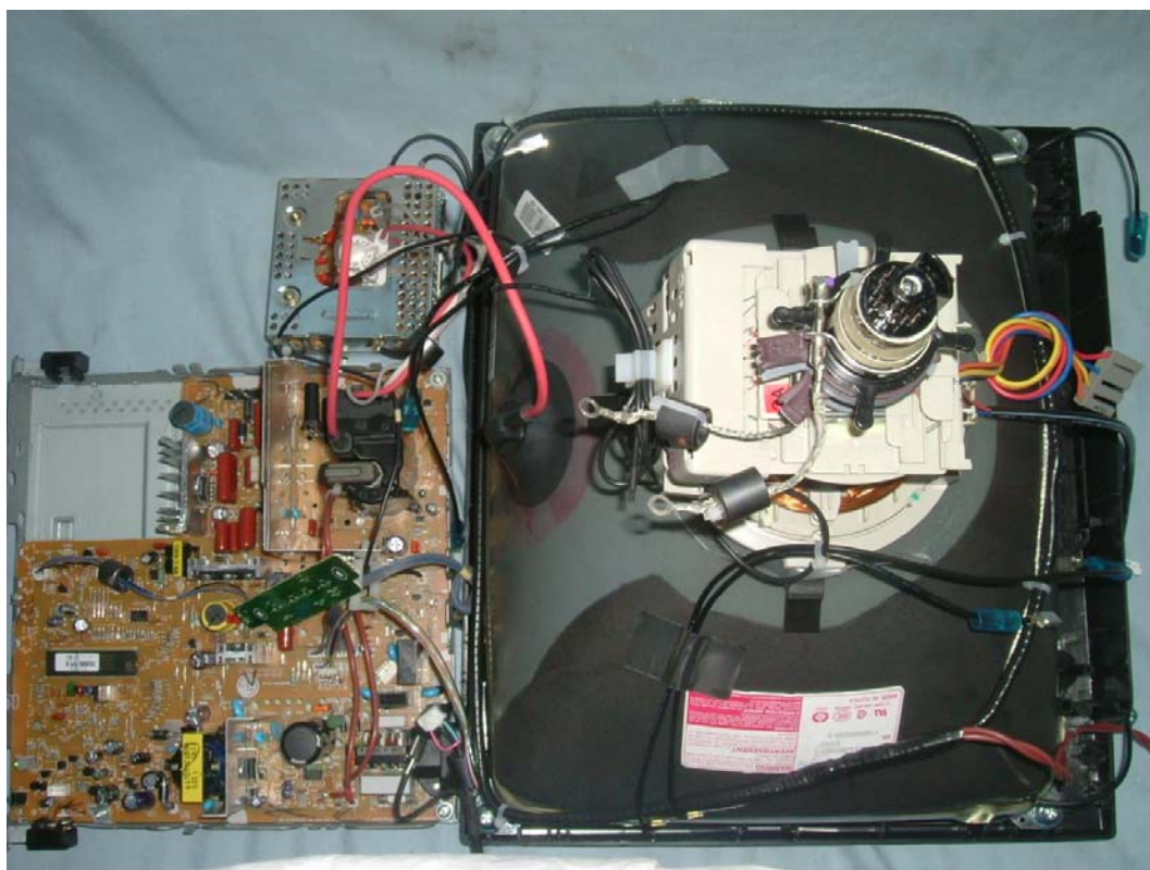
FIGURE 7 CRT MONITOR (M/N: C17PC-*) BOARD REMOVED
