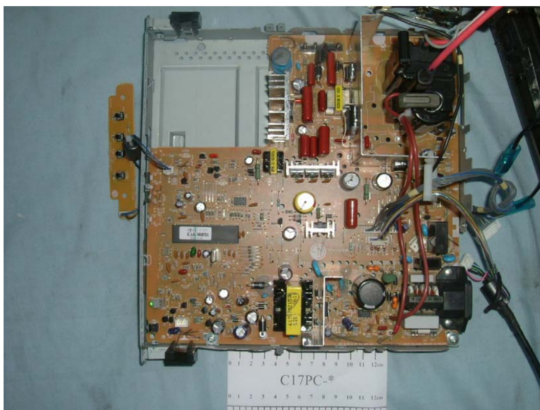
FIGURE 9 CRT MONITOR (M/N: C17PC-*) MAIN BOARD 1
