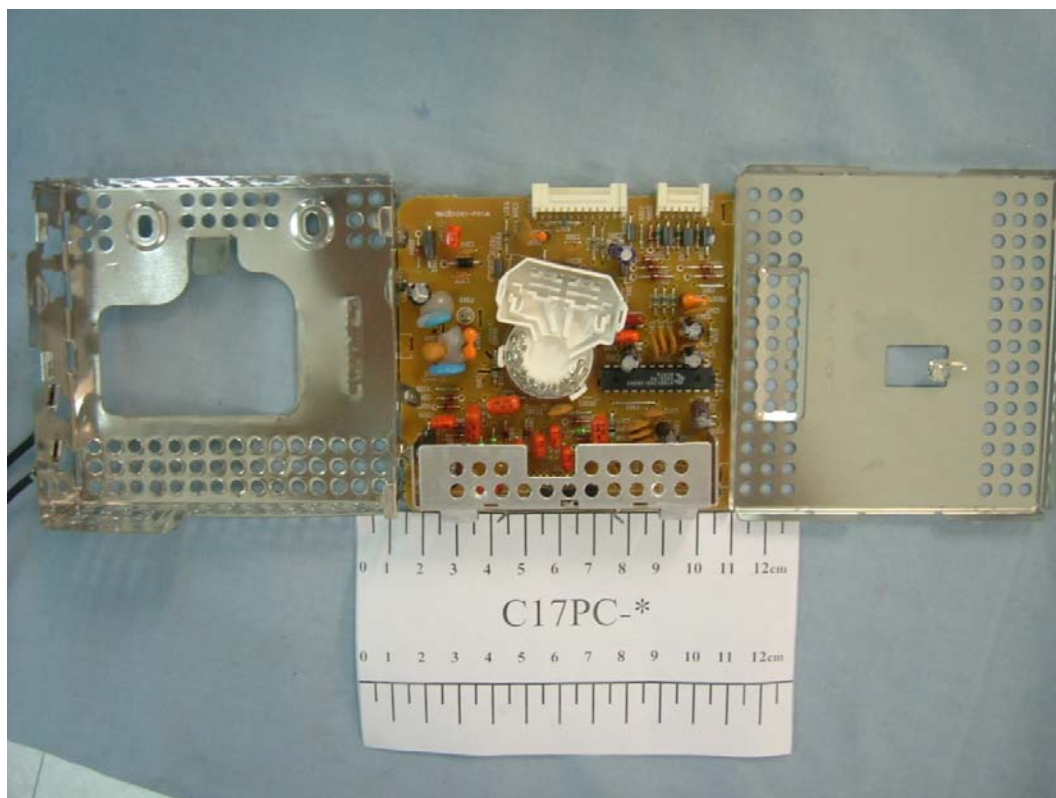
FIGURE 16 CRT MONITOR (M/N: C17PC-*) MAIN BOARD 2 COVER REMOVED
