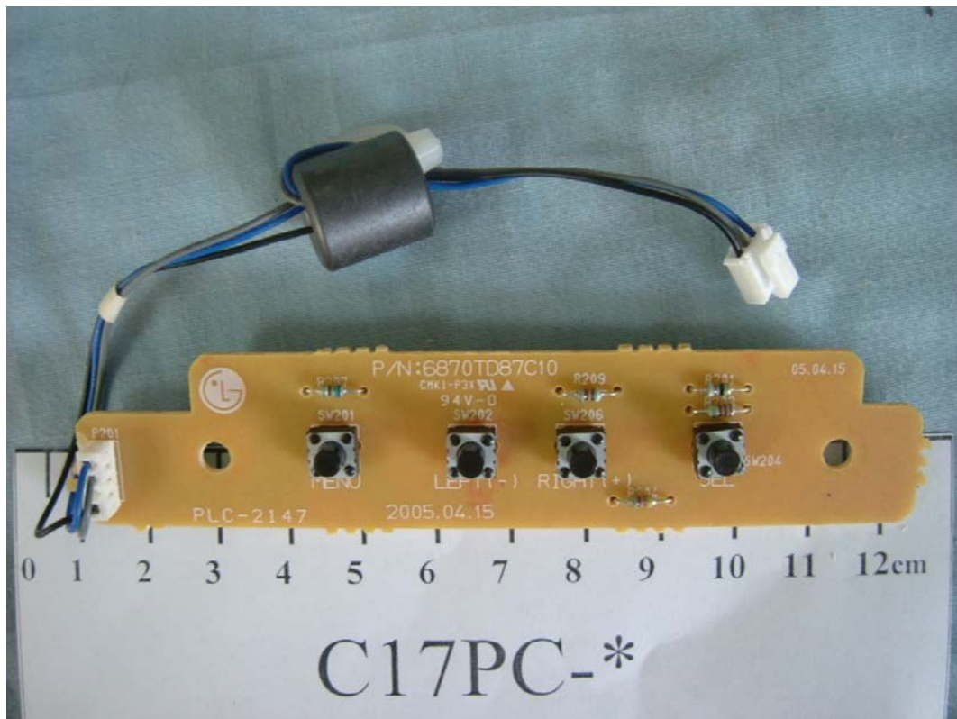
FIGURE 13 CRT MONITOR (M/N: C17PC-*) BUTTON CONTROL BOARD (COMPONENT SIDE)
