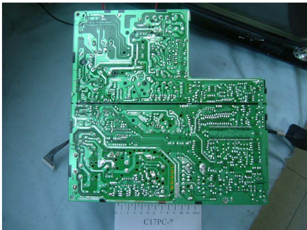
FIGURE 12 CRT MONITOR (M/N: C17PC-*) MAIN BOARD 1 (SOLDERED SIDE)
