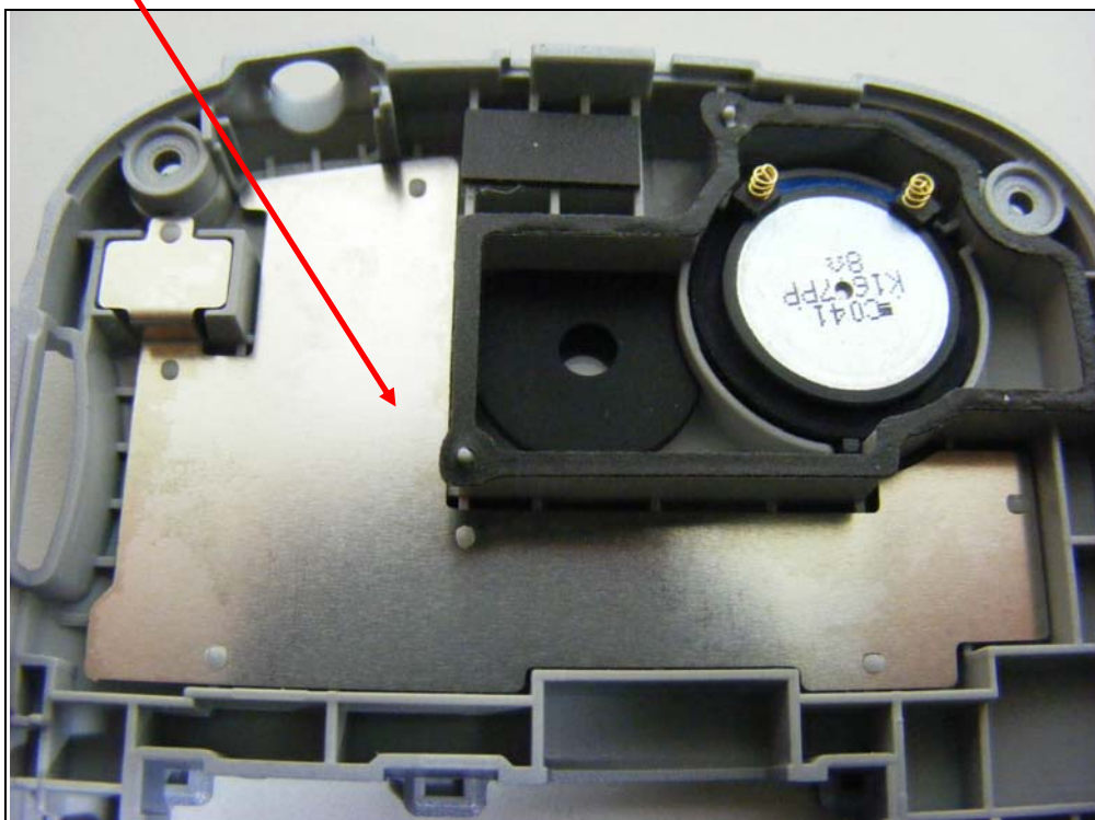
FM Radio Antenna
