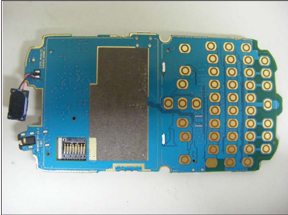
Top view of Main PCB (Removing LCD and Dome sheet)
