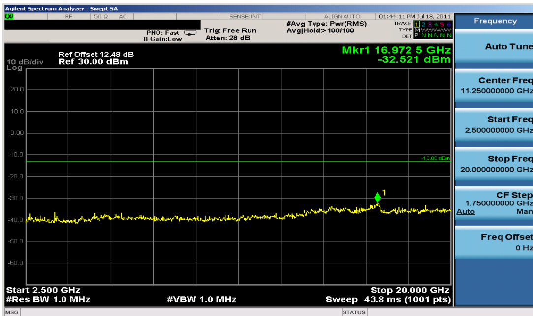
Plot 7-35. Conducted Spurious Plot (PCS WCDMA Mode – Ch. 9262)
