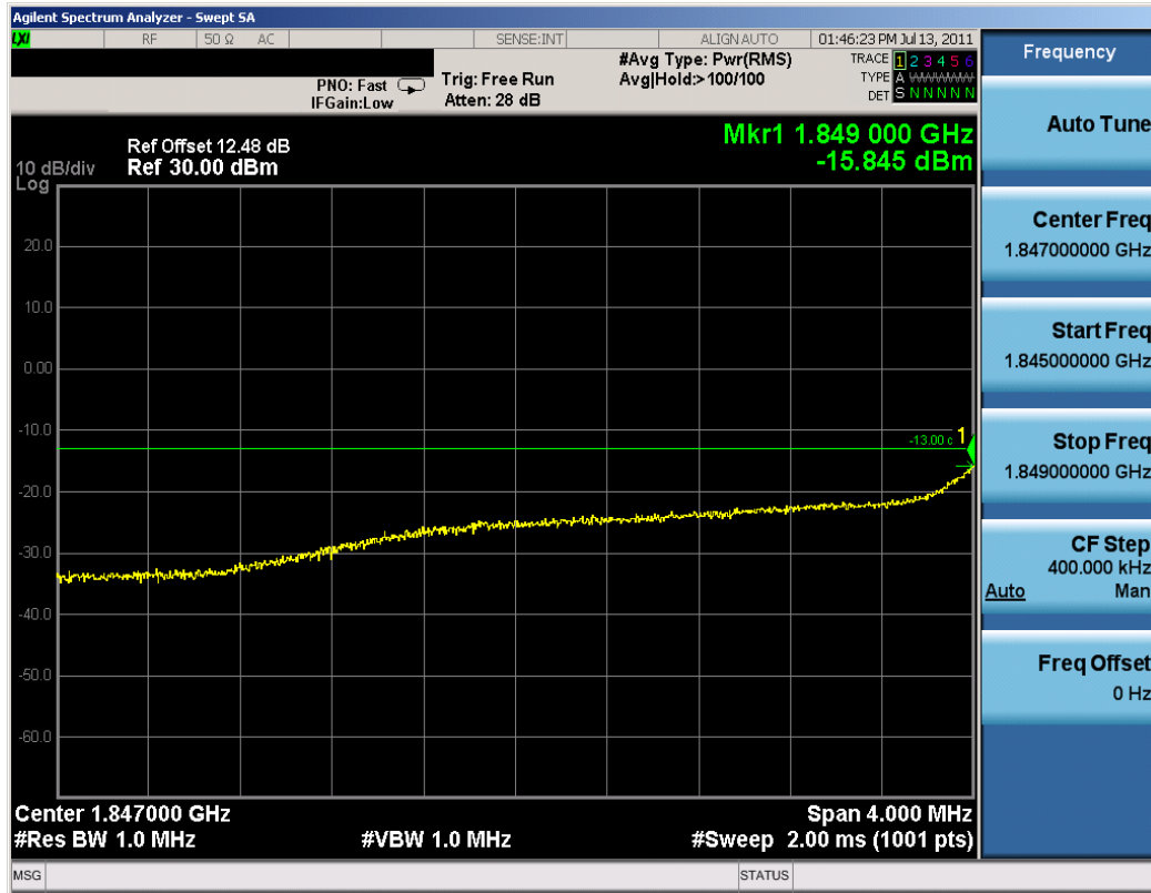
Plot 7-37. 4MHz Span Plot (PCS WCDMA Mode – Ch. 9262)
