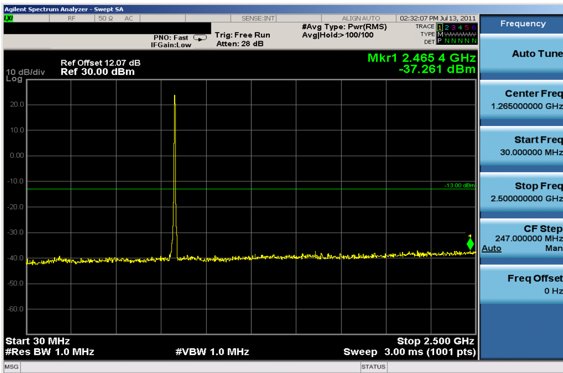
Plot 7-30. Conducted Spurious Plot (Cellular WCDMA Mode – Ch. 4233)
