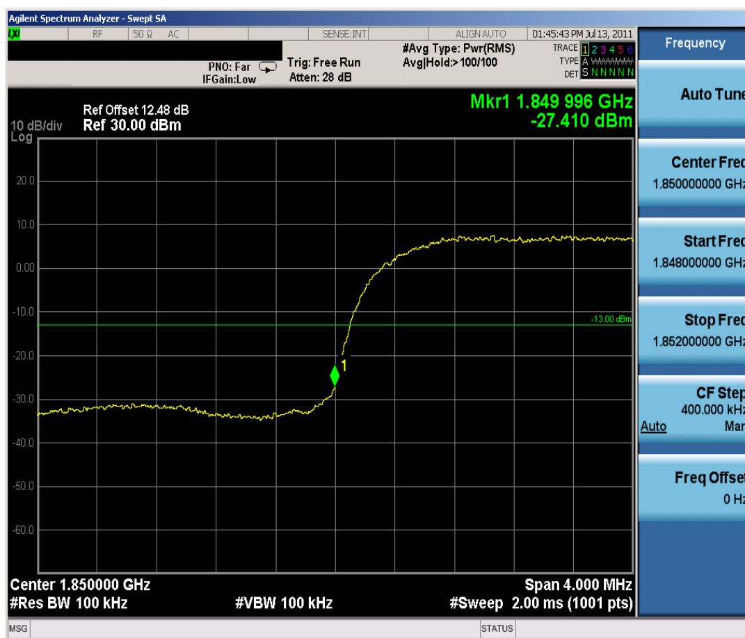
Plot 7-36. Band Edge Plot (PCS WCDMA Mode – Ch. 9262)
