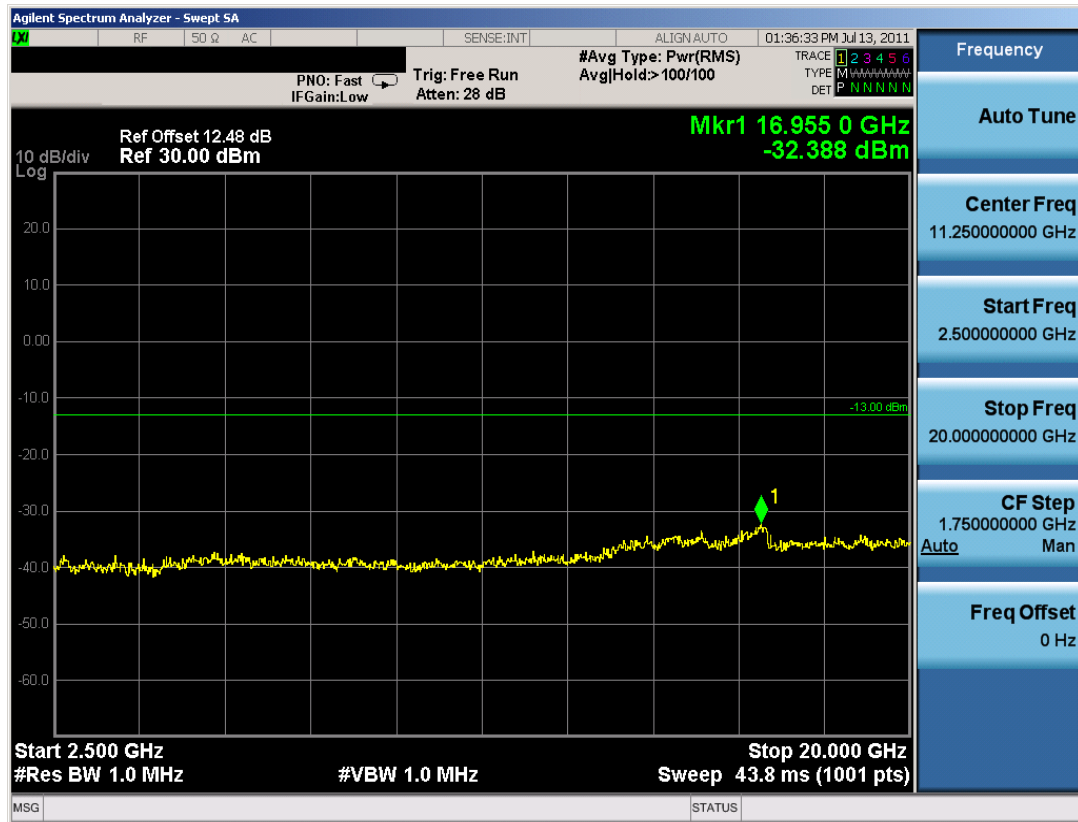
Plot 7-39. Conducted Spurious Plot (PCS WCDMA Mode – Ch. 9400)
