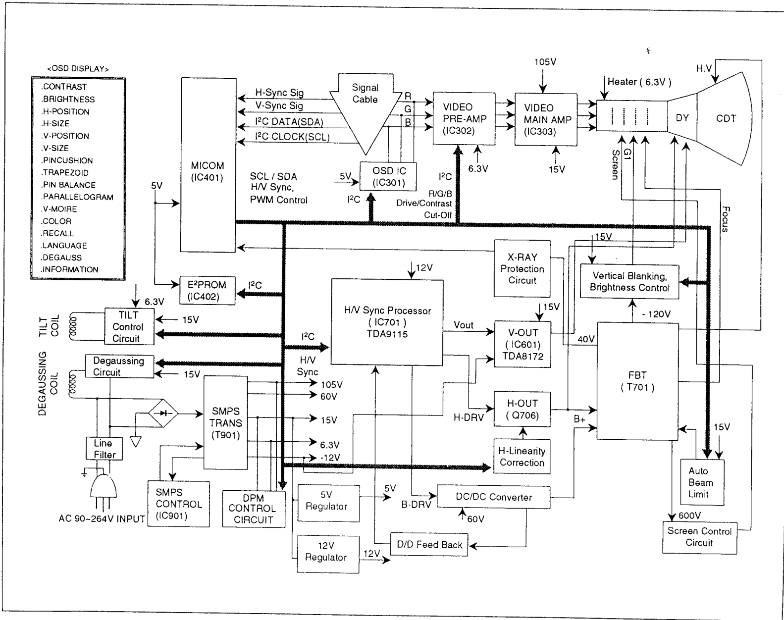
BLOCK DIAGRAM
