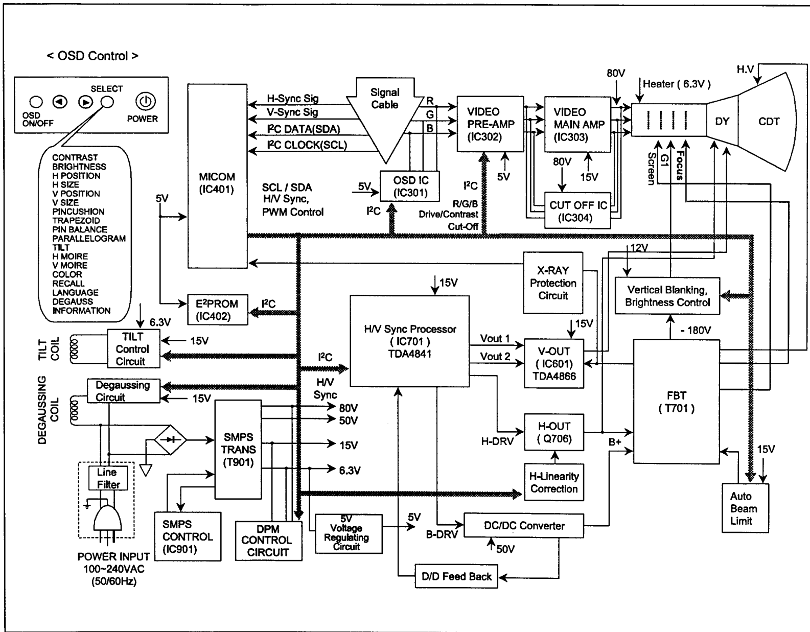
BLOCK DIAGRAM
