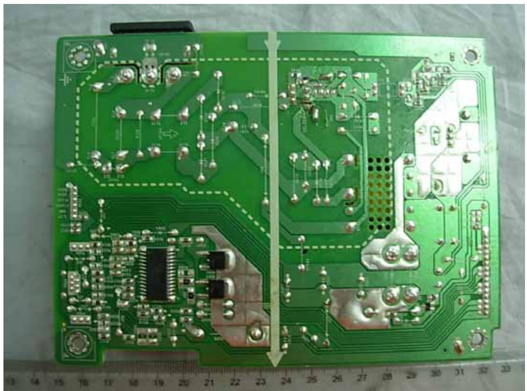
FIGURE 4 LCD MONITOR (M/N: D2341PY) POWER BOARD (COMPONENT SIDE)
