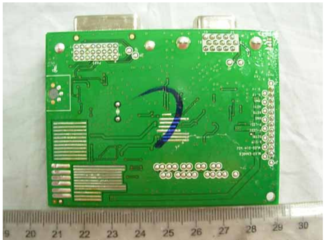
FIGURE 6 LCD MONITOR (M/N: D2341PY) MAIN BOARD (SOLDERED SIDE)
