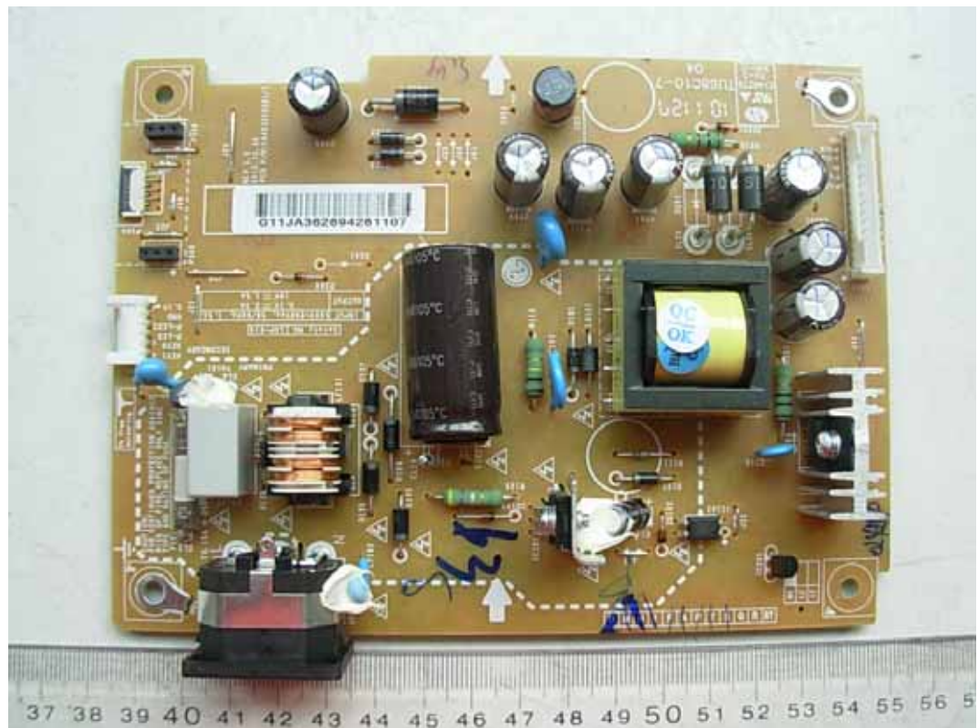
FIGURE 6 LCD MONITOR (M/N: D2342PY) POWER BOARD (COMPONENT SIDE)
