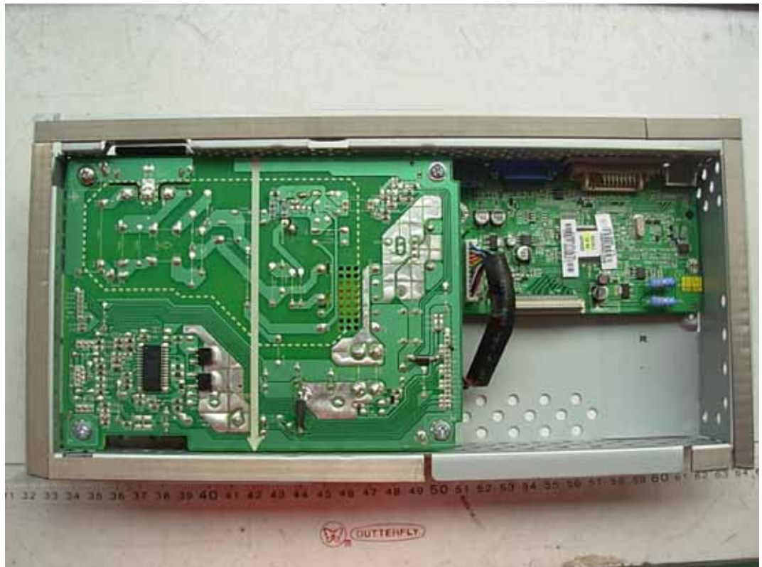
FIGURE 14 LCD MONITOR (M/N: D2342PY) DEBUG #3
