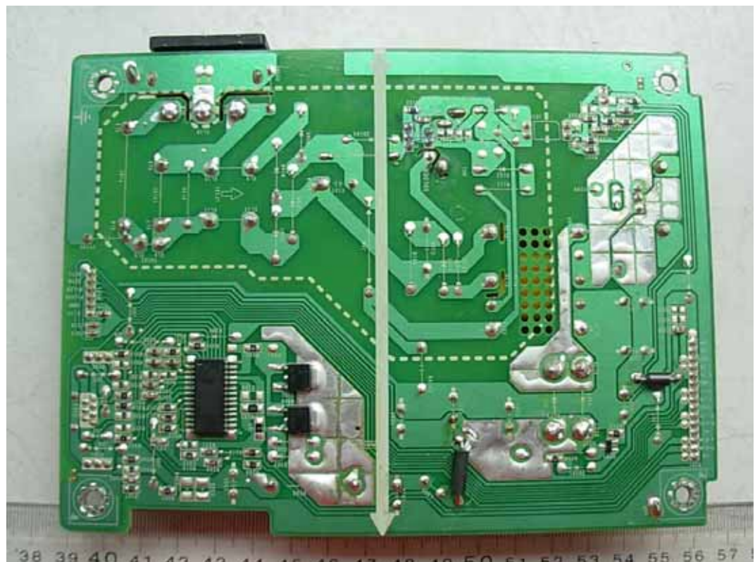
FIGURE 7 LCD MONITOR (M/N: D2342PY) POWER BOARD (SOLDERED SIDE)
