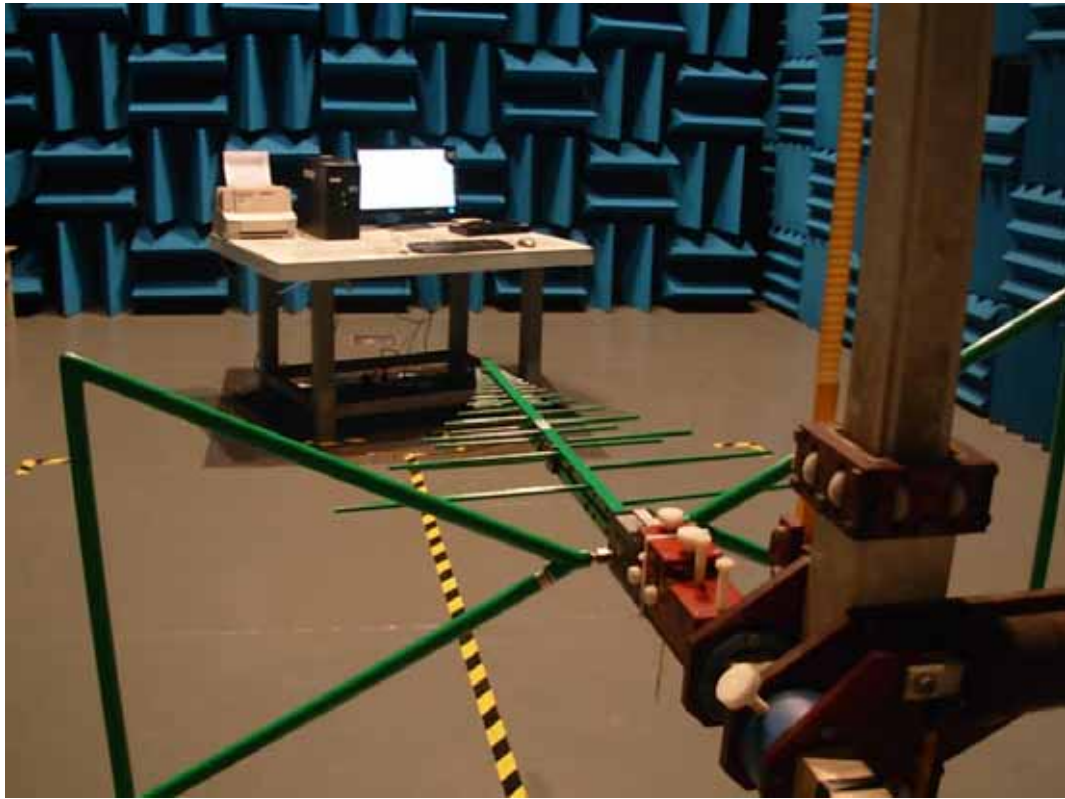
SETUP WITH MAXIMUM DETECTED EMISSION AT HORIZONTAL POLARIZATION (TEST MODE: DVI 1280*1024@60Hz)
