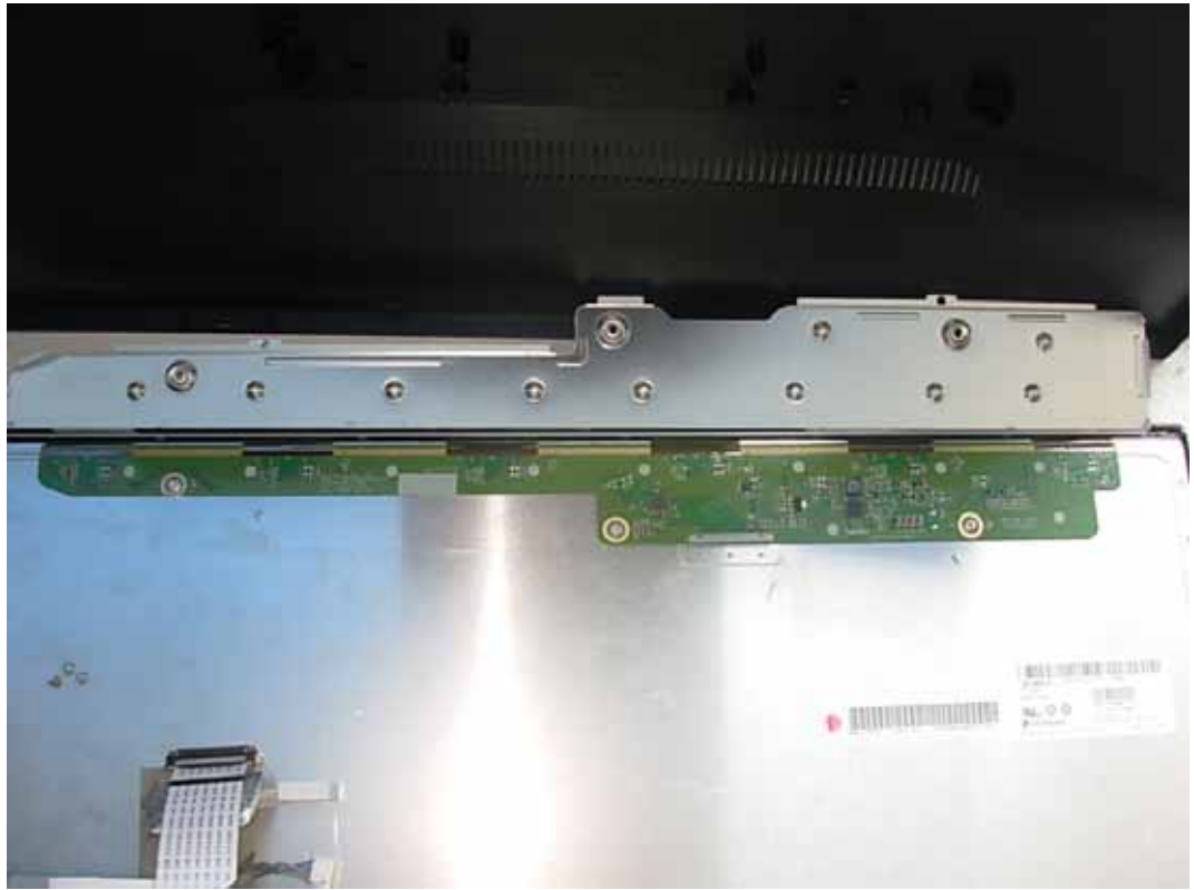
FIGURE 8 LCD MONITOR (M/N: D2542PY) DISPLAY BOARD (COMPONENT SIDE)
