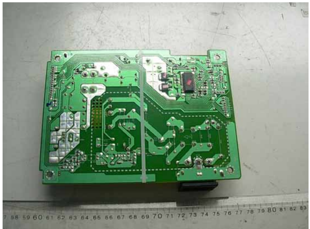
FIGURE 7 LCD MONITOR (M/N: D2542PY) POWER BOARD (SOLDERED SIDE)
