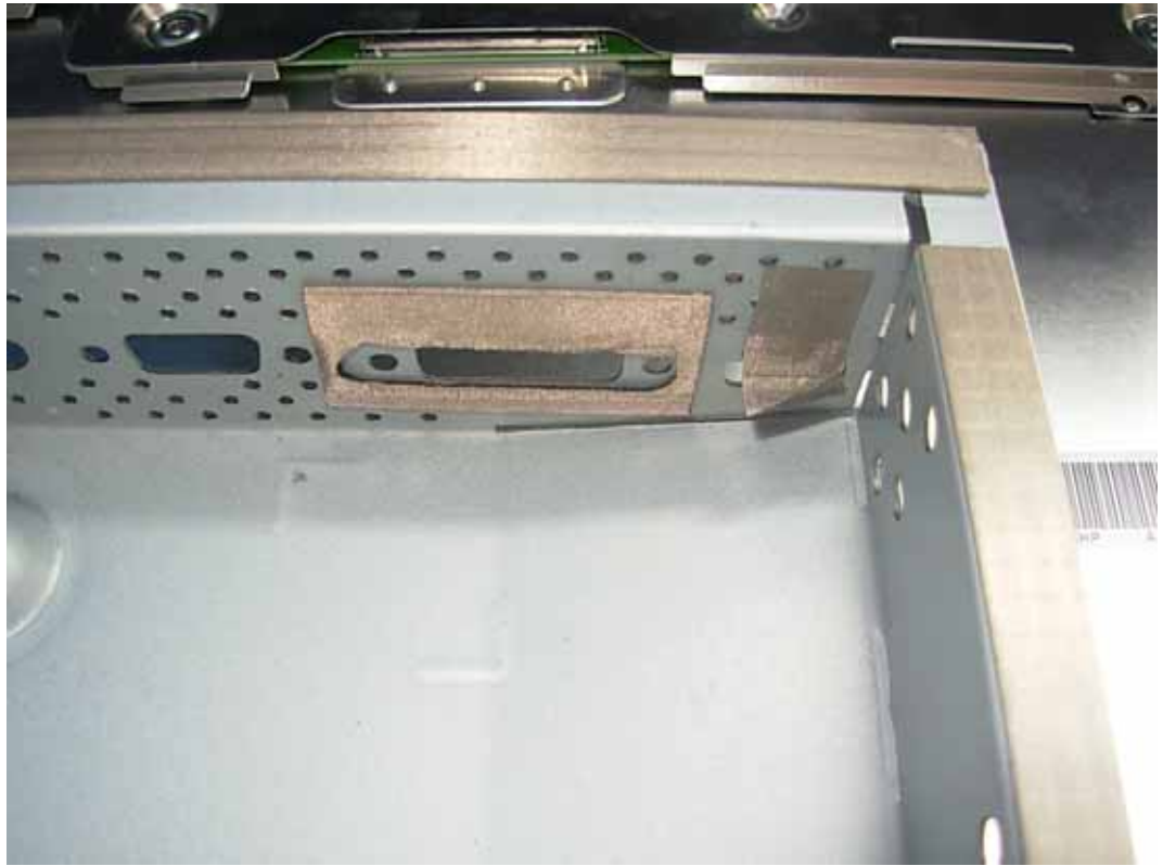
FIGURE 14 LCD MONITOR (M/N: D2542PY) DEBUG #3
