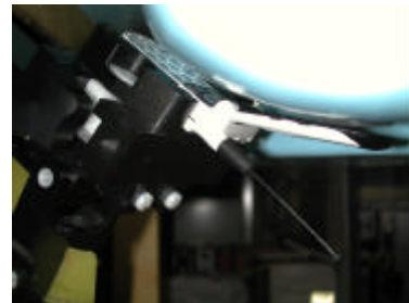
Figure 18. Head SAR Test Setup
