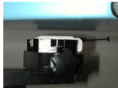
Figure 19. Body SAR Test Setup
