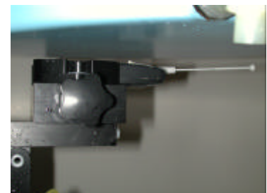
Figure 20. Body SAR Test Setup
