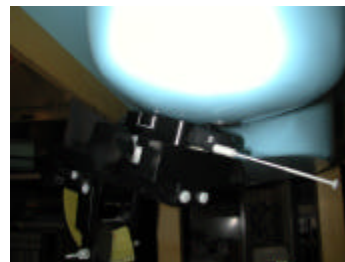
Figure 18. Head SAR Test Setup
