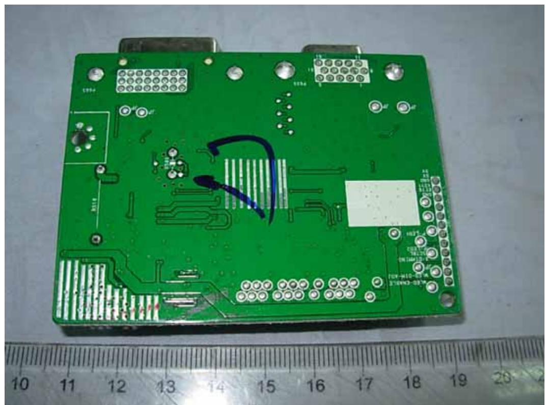
FIGURE 6 LCD MONITOR (M/N: E1910PW) MAIN BOARD (SOLDERED SIDE)
