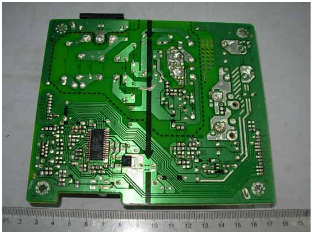
FIGURE 4 LCD MONITOR (M/N: E1910PW) POWER BOARD (COMPONENT SIDE)
