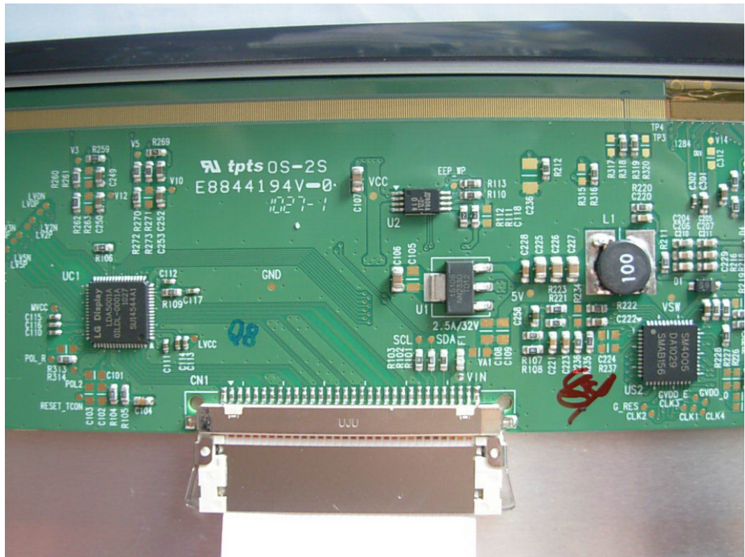
FIGURE 6 LCD MONITOR (M/N: E1910SW) CHIPS ON PANEL BOARD
