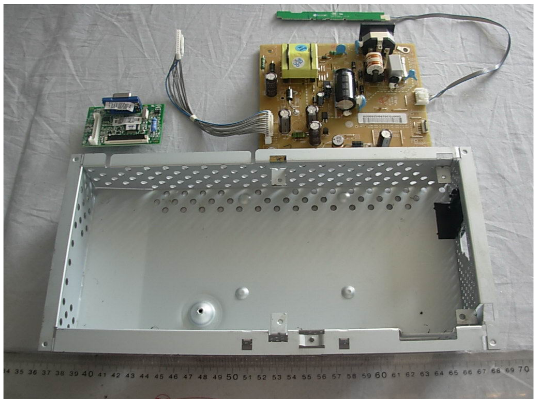
FIGURE 7 LCD MONITOR (M/N: E1910SW) BOARDS REMOVED
