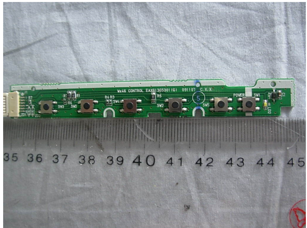
FIGURE 13 LCD MONITOR (M/N: E1910SW) BUTTON BOARD (COMPONENT SIDE)
