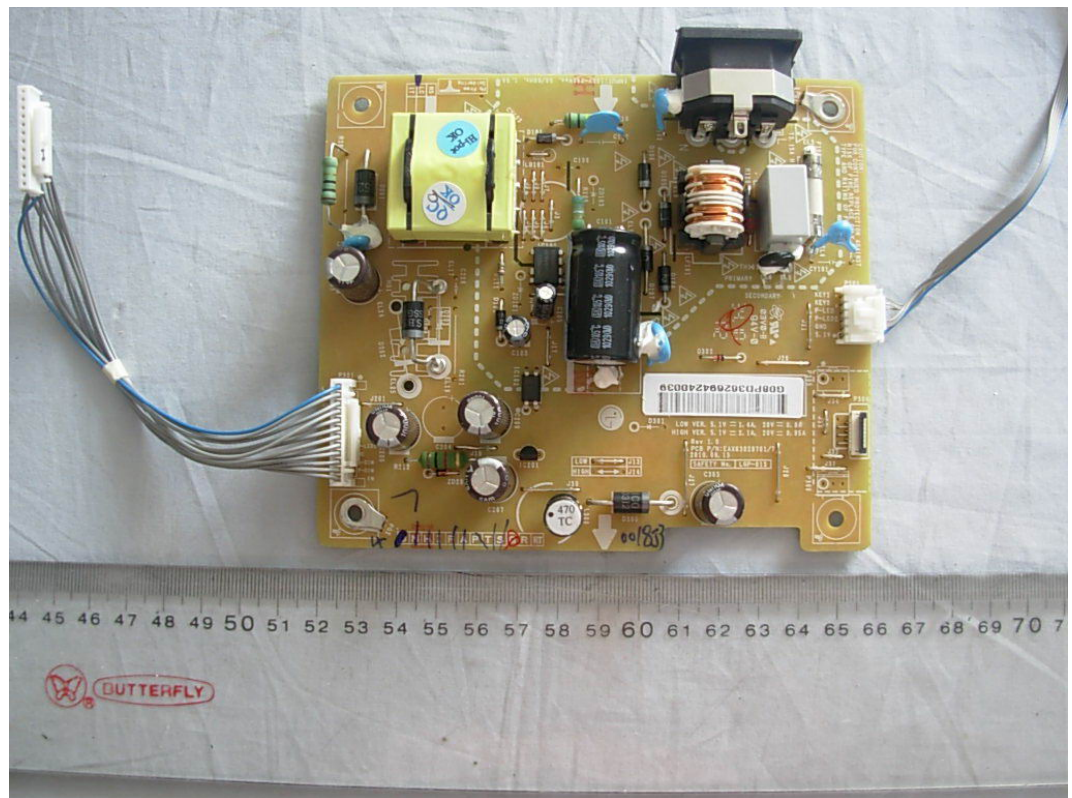
FIGURE 8 LCD MONITOR (M/N: E1910SW) POWER BOARD (COMPONENT SIDE)
