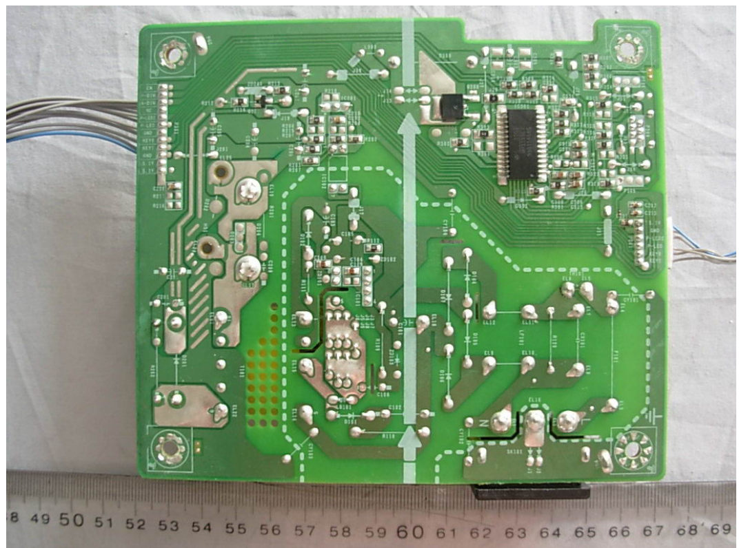
FIGURE 9 LCD MONITOR (M/N: E1910SW) POWER BOARD (SOLDERED SIDE)
