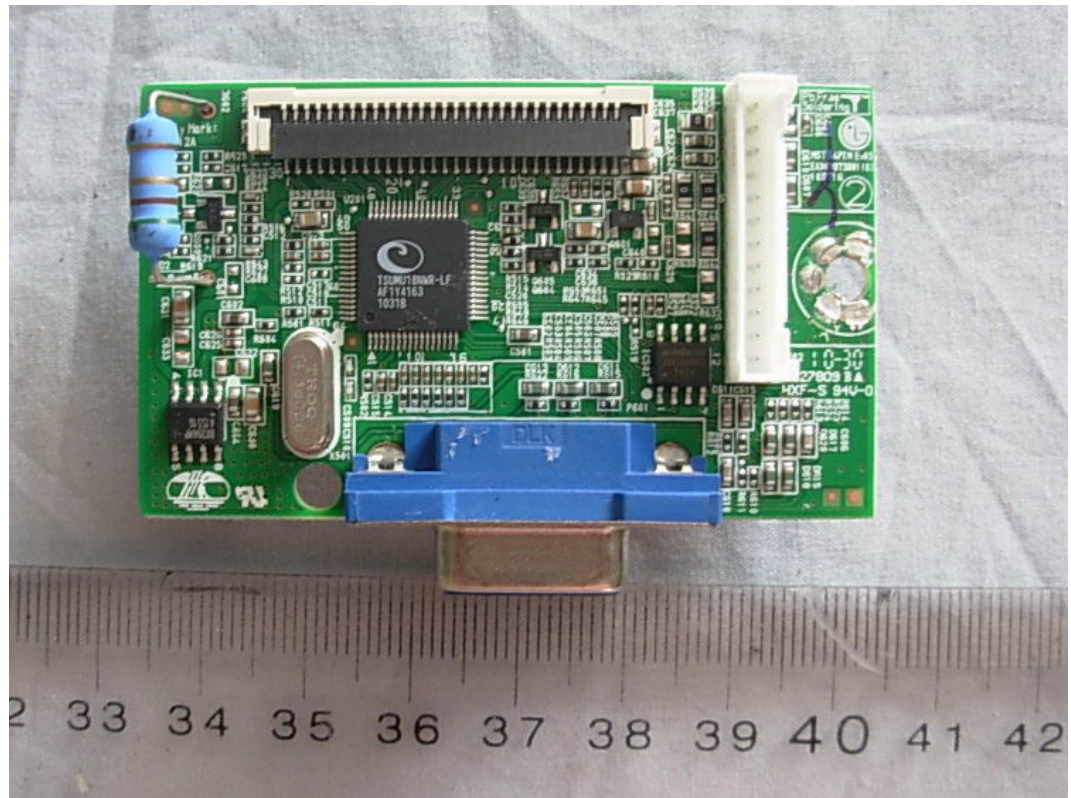
FIGURE 10 LCD MONITOR (M/N: E1910SW) MAIN BOARD (COMPONENT SIDE)
