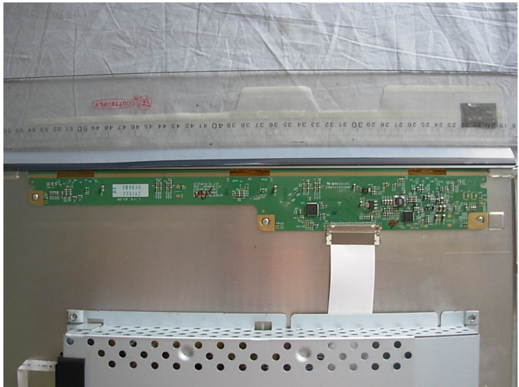
FIGURE 4 LCD MONITOR (M/N: E1910SW) PANEL BOARD (COMPONENT SIDE)
