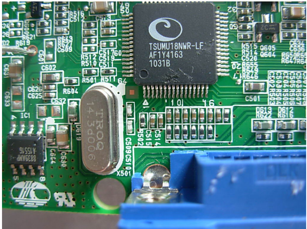
FIGURE 12 LCD MONITOR (M/N: E1910SW) CHIP & CRYSTAL ON MAIN BOARD
