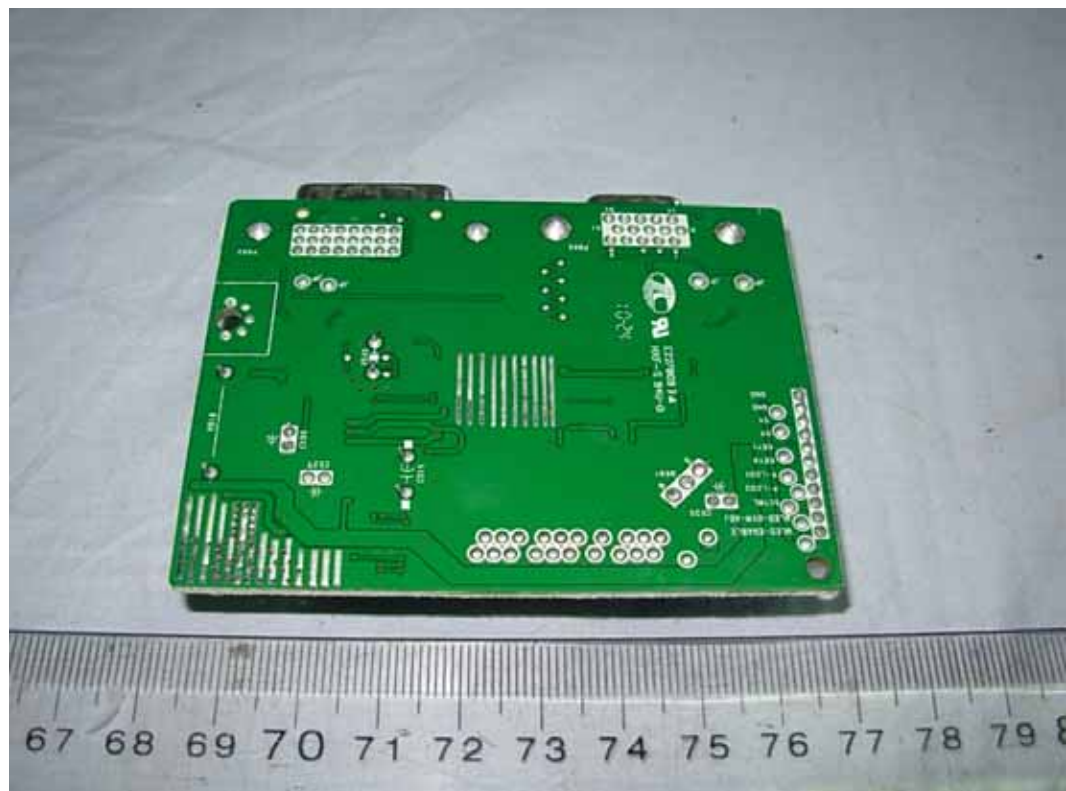
FIGURE 6 LCD MONITOR (M/N: E1910TW) MAIN BOARD (SOLDERED SIDE)
