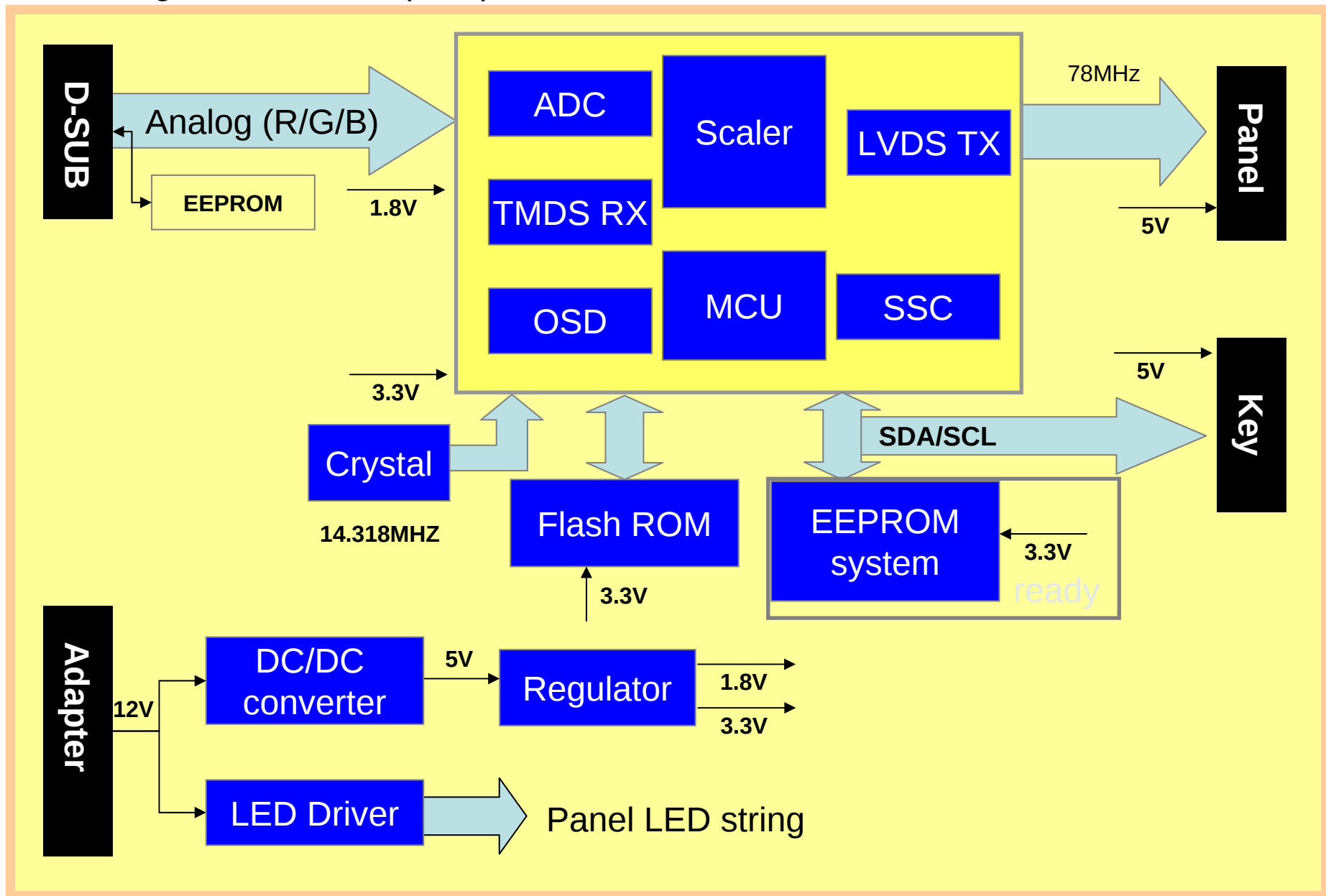
Block diagram for E1940 (NVT)
