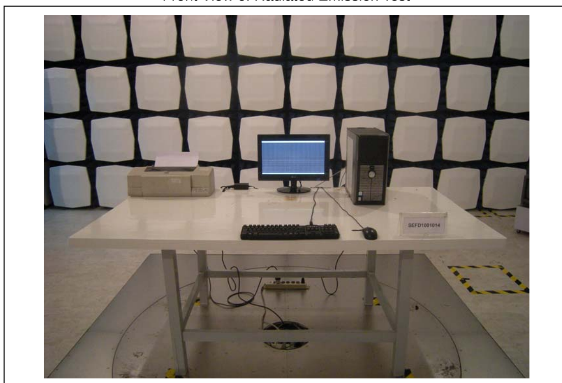
Front View of Radiated Emission Test
