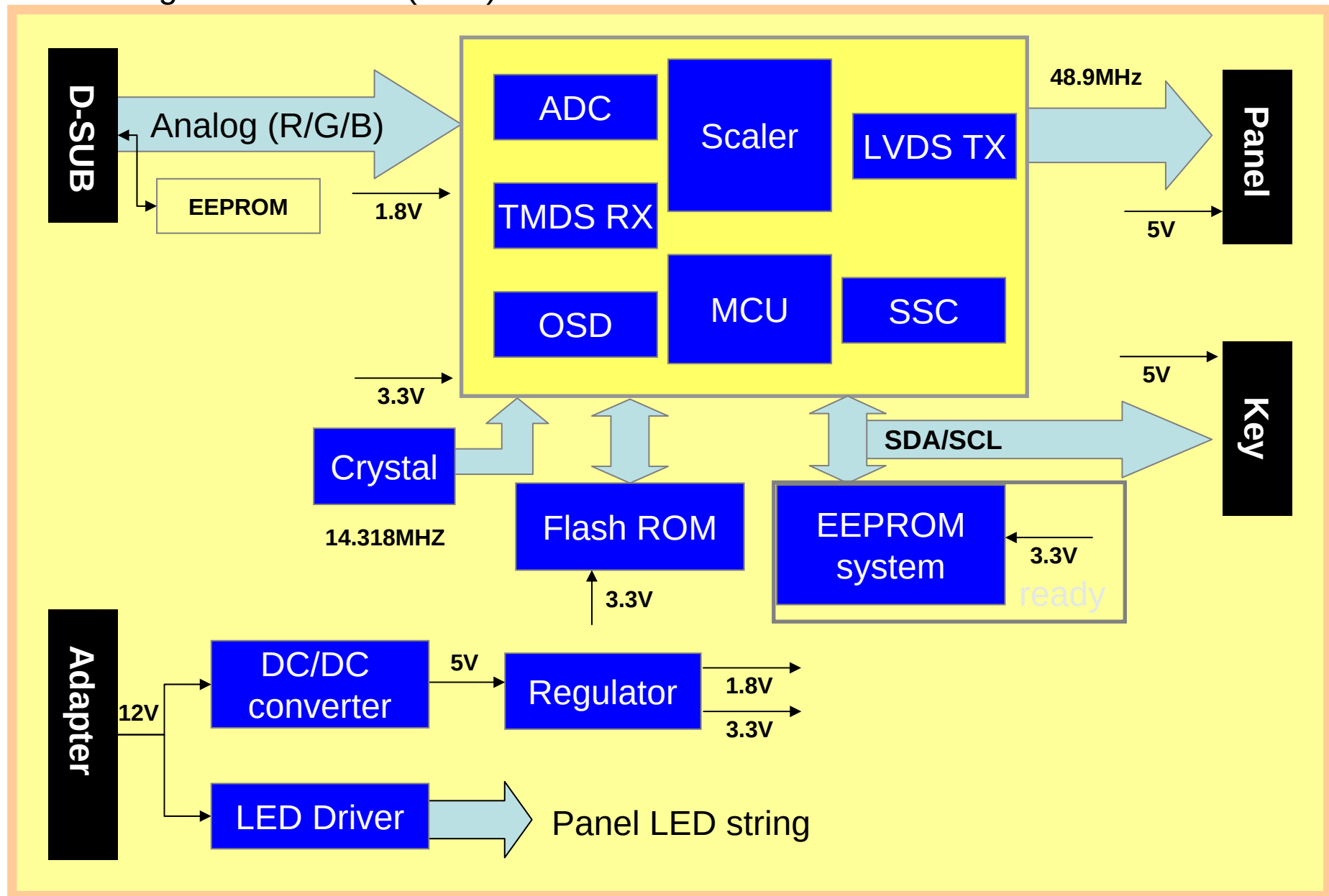
Block diagram for E2040 (NVT)
