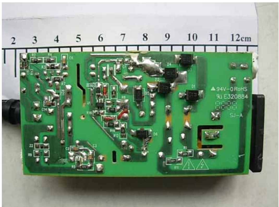
FIGURE 11 LCD MONITOR (M/N: E2050SV) ADAPTER #1 (MAIN BOARD – SOLDERED SIDE)
