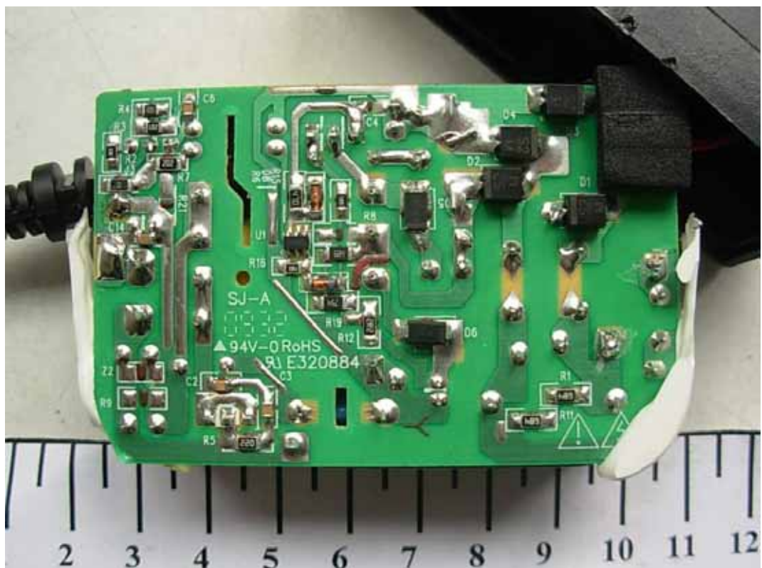
FIGURE 16 LCD MONITOR (M/N: E2050SV) ADAPTER #2 (MAIN BOARD – SOLDERED SIDE)
