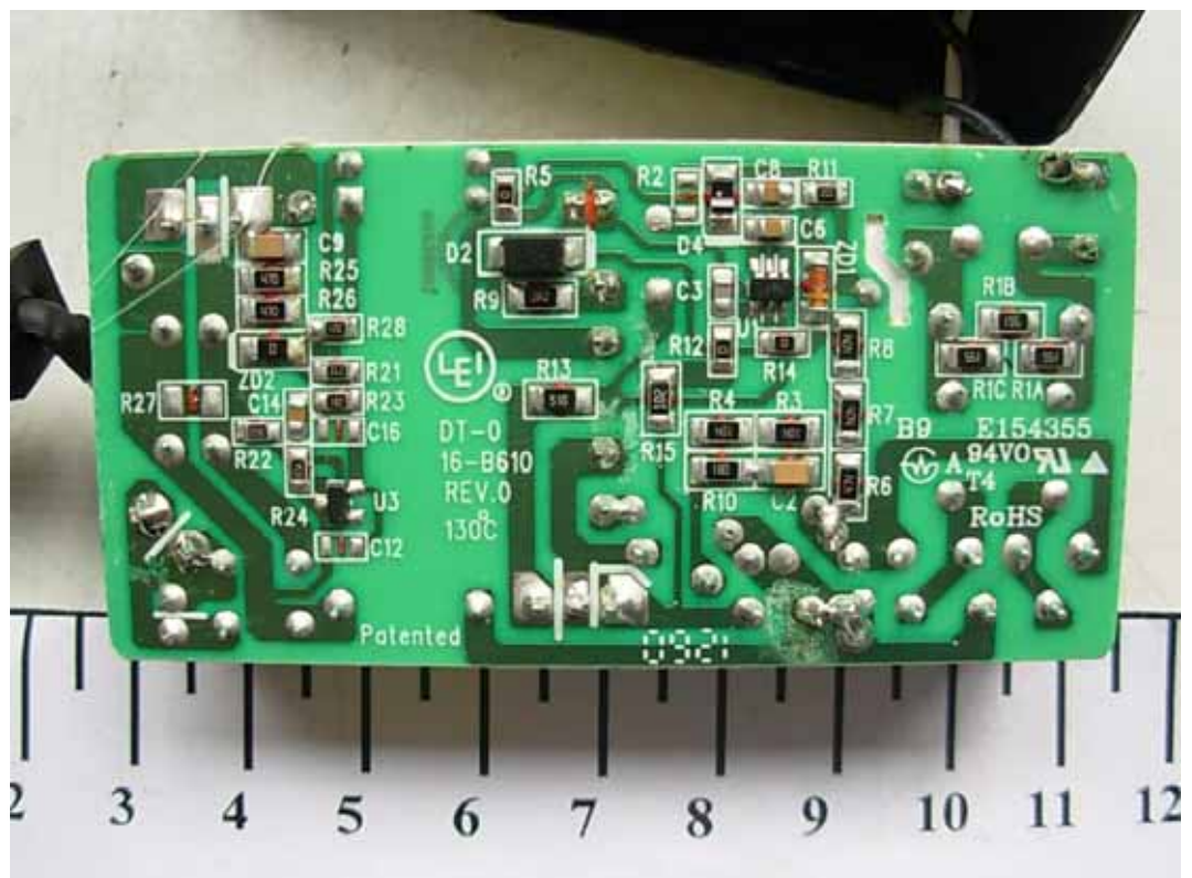
FIGURE 27 LCD MONITOR (M/N: E2050SV) ADAPTER #4 (MAIN BOARD – SOLDERED SIDE)
