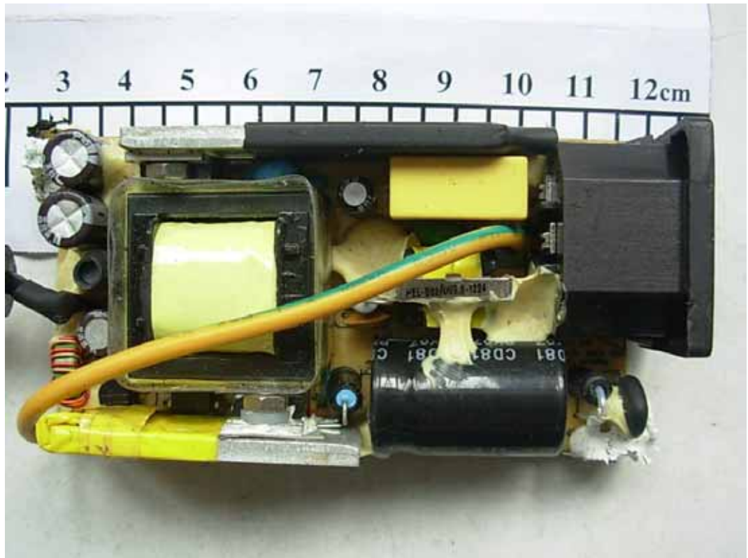
FIGURE 10 LCD MONITOR (M/N: E2050SV) ADAPTER #1 (MAIN BOARD – COMPONENT SIDE)
