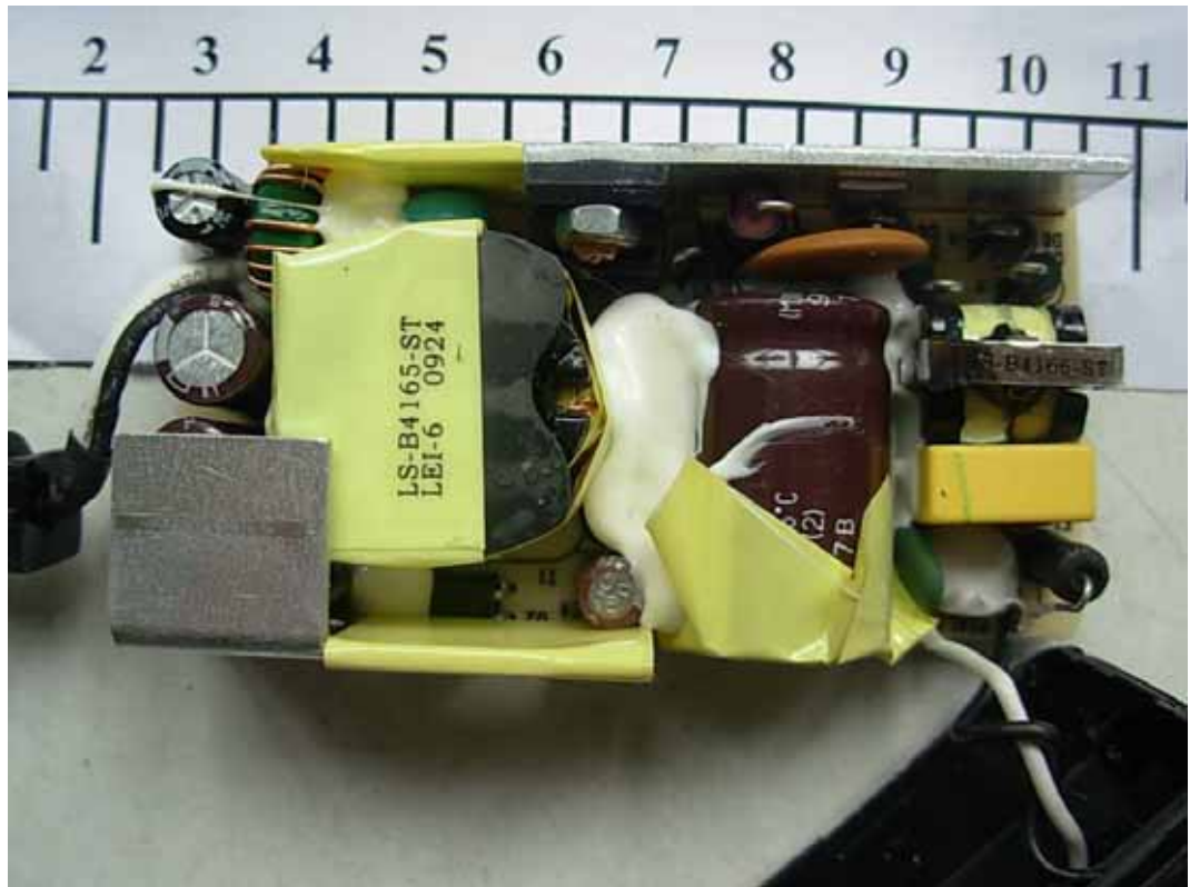
FIGURE 26 LCD MONITOR (M/N: E2050SV) ADAPTER #4 (MAIN BOARD – COMPONENT SIDE)
