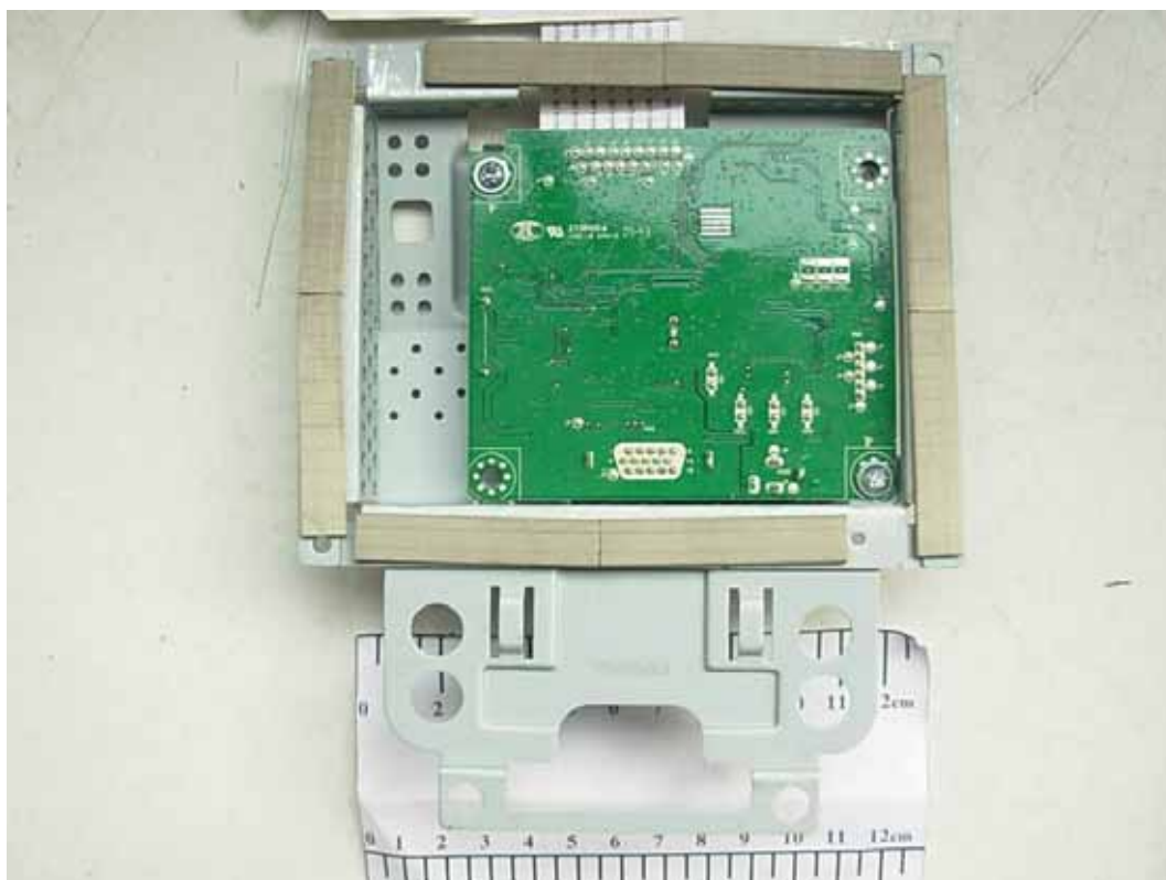
FIGURE 11 LCD MONITOR (M/N: E2050SV) DEBUG #2
