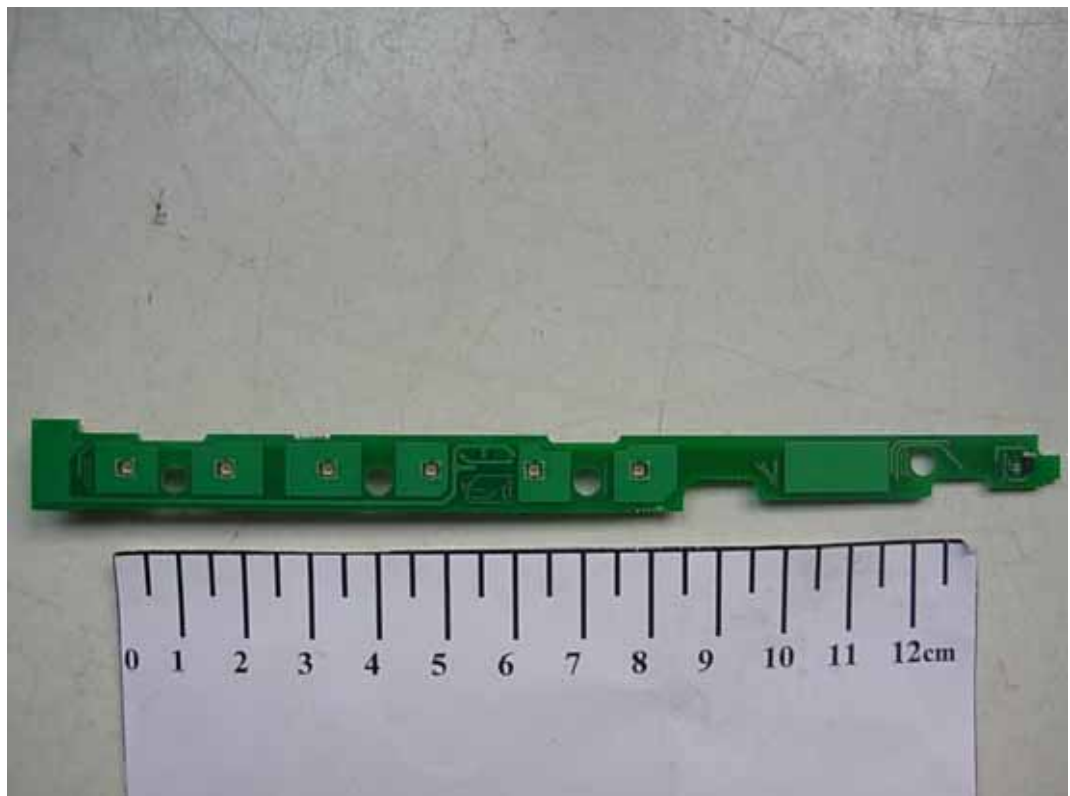
FIGURE 6 LCD MONITOR (M/N: E2050SV) KEY BOARD (SOLDERED SIDE)
