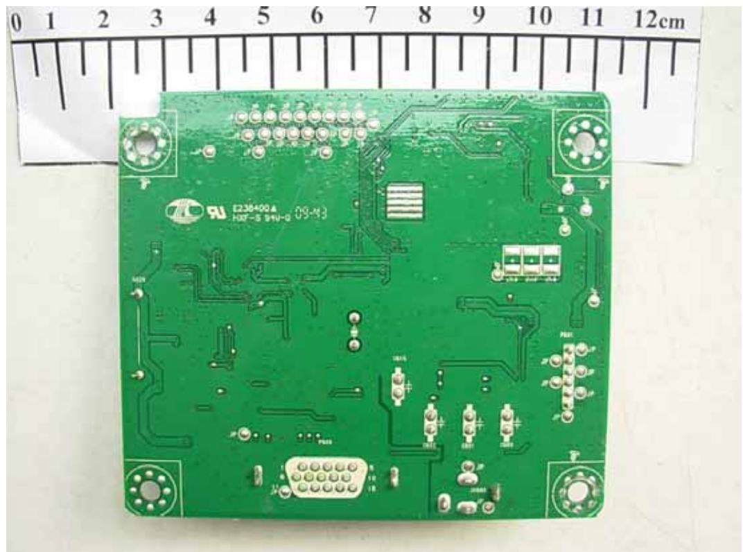
FIGURE 3 LCD MONITOR (M/N: E2050SV) MAIN BOARD (SOLDERED SIDE)
