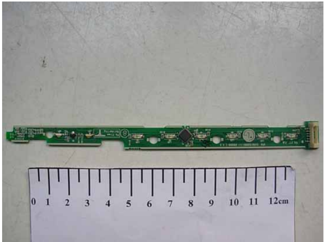
FIGURE 5 LCD MONITOR (M/N: E2050SV) KEY BOARD (COMPONENT SIDE)
