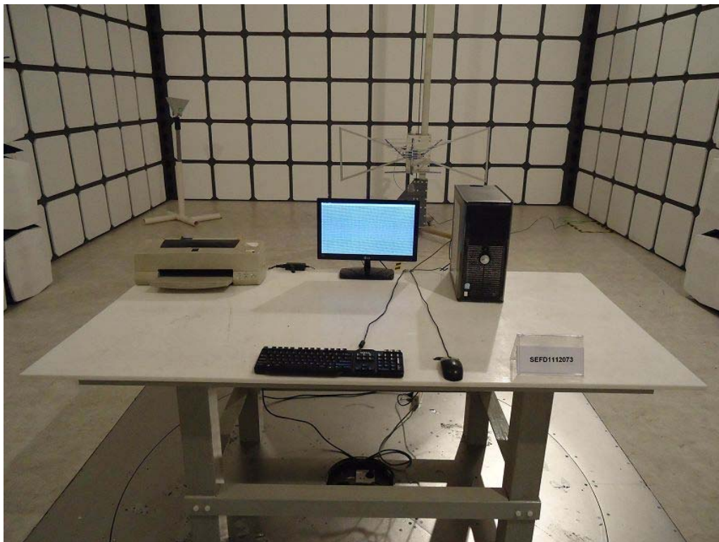
Front View of Radiated Emission Test (30MHz ~ 1000MHz)
