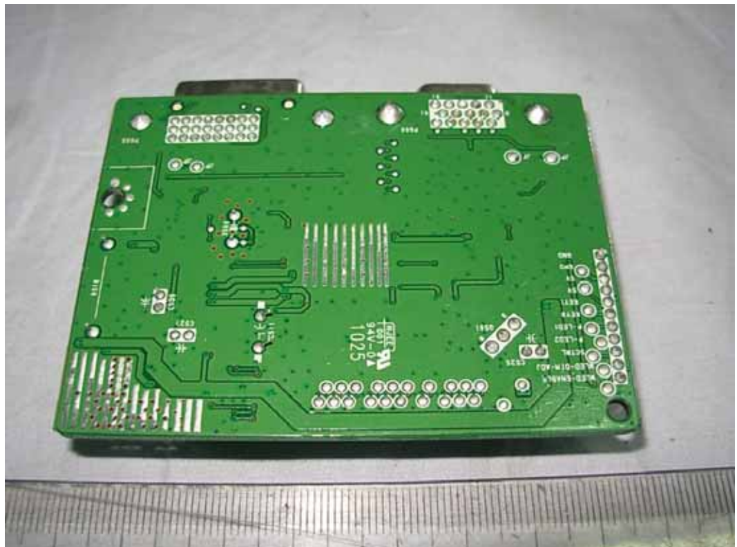
FIGURE 6 LCD MONITOR (M/N: E2210TW) MAIN BOARD (SOLDERED SIDE)
