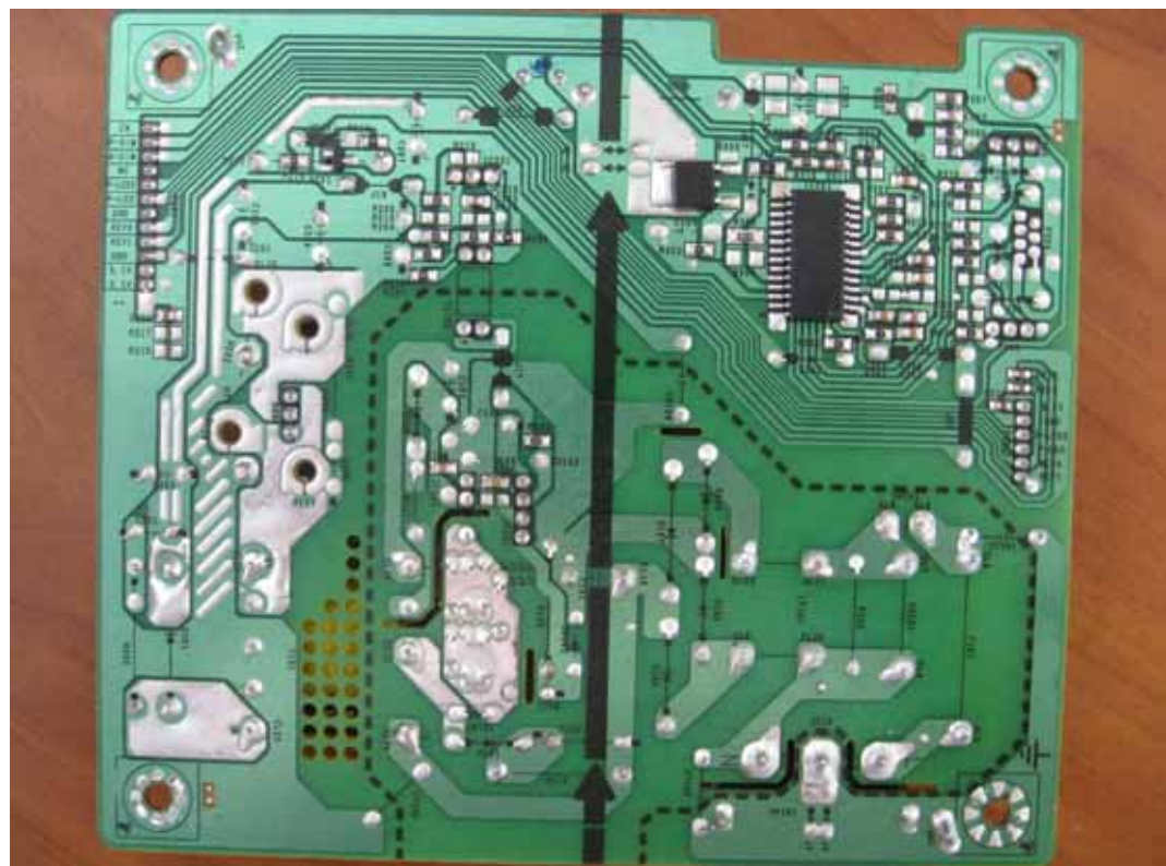
FIGURE 4 LCD MONITOR (M/N: E2210TW) POWER BOARD (SOLDERED SIDE)
