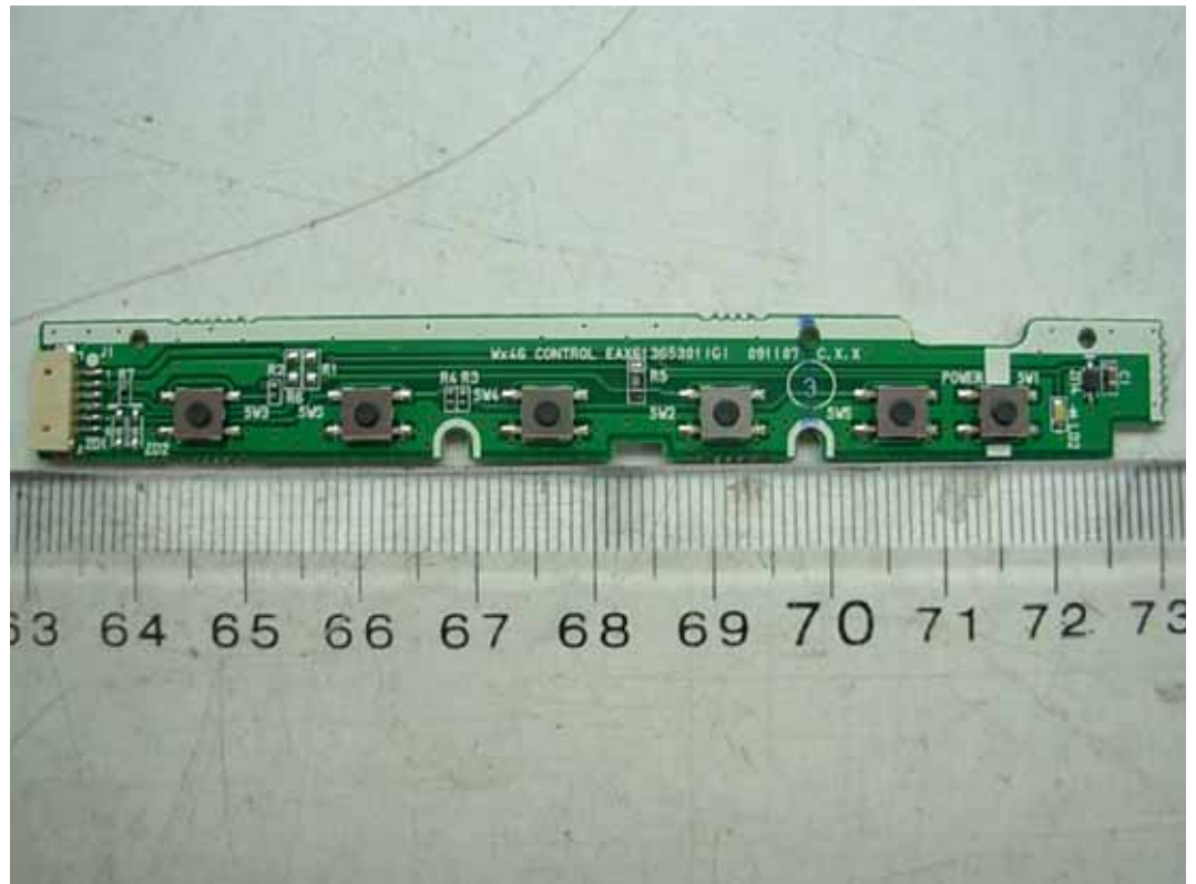
FIGURE 10 LCD MONITOR (M/N: E2211TX) KEY BOARD (COMPONENT SIDE)
