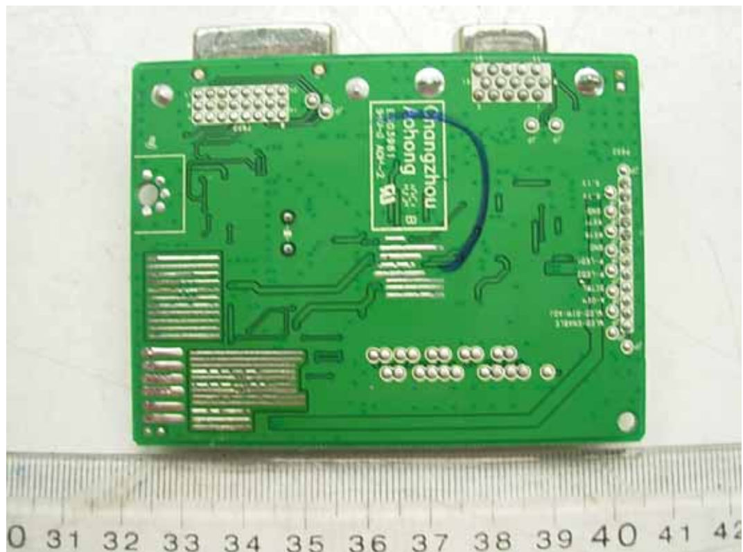
FIGURE 6 LCD MONITOR (M/N: E2211TX) MAIN BOARD (SOLDERED SIDE)
