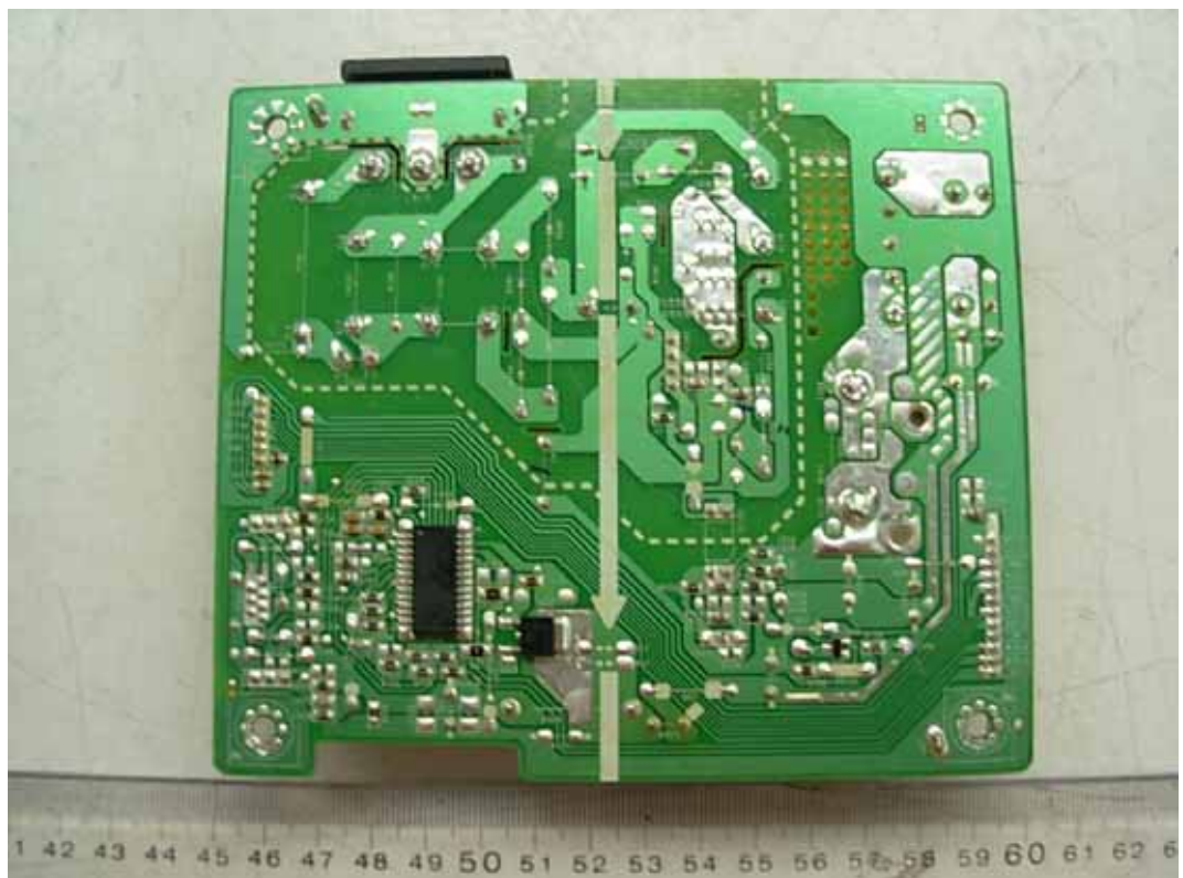
FIGURE 4 LCD MONITOR (M/N: E2211TX) POWER BOARD (COMPONENT SIDE)
