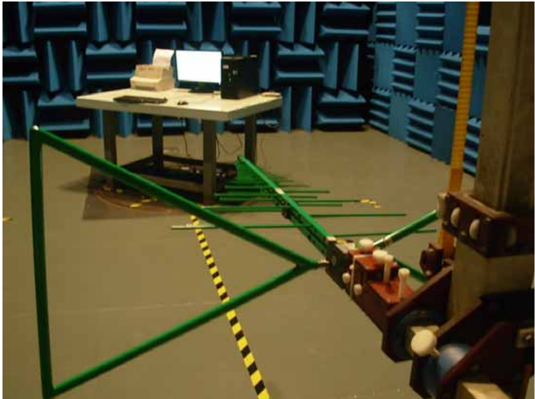
SETUP WITH MAXIMUM DETECTED EMISSION AT HORIZONTAL POLARIZATION (TEST MODE: DVI 1680*1050@60Hz)
