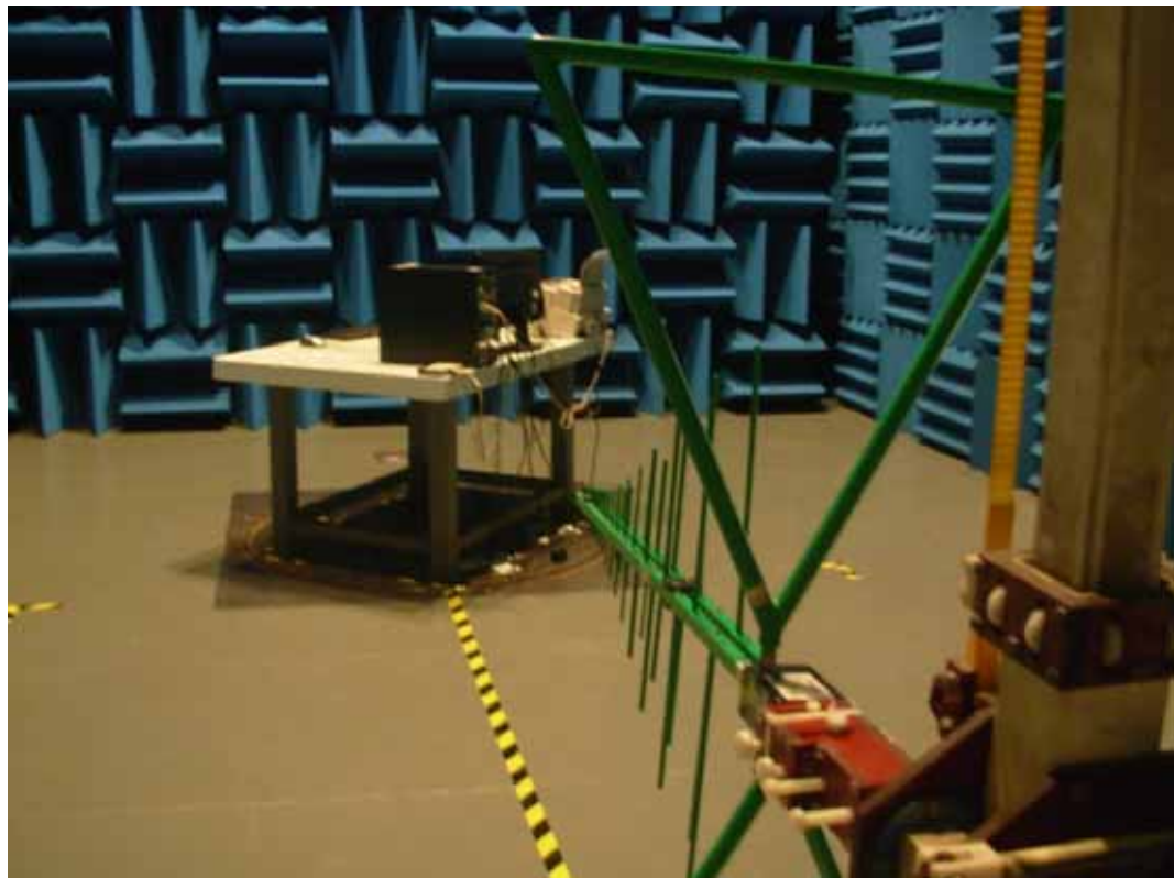
SETUP WITH MAXIMUM DETECTED EMISSION AT VERTICAL POLARIZATION (TEST MODE: DVI 1680*1050@60Hz)
