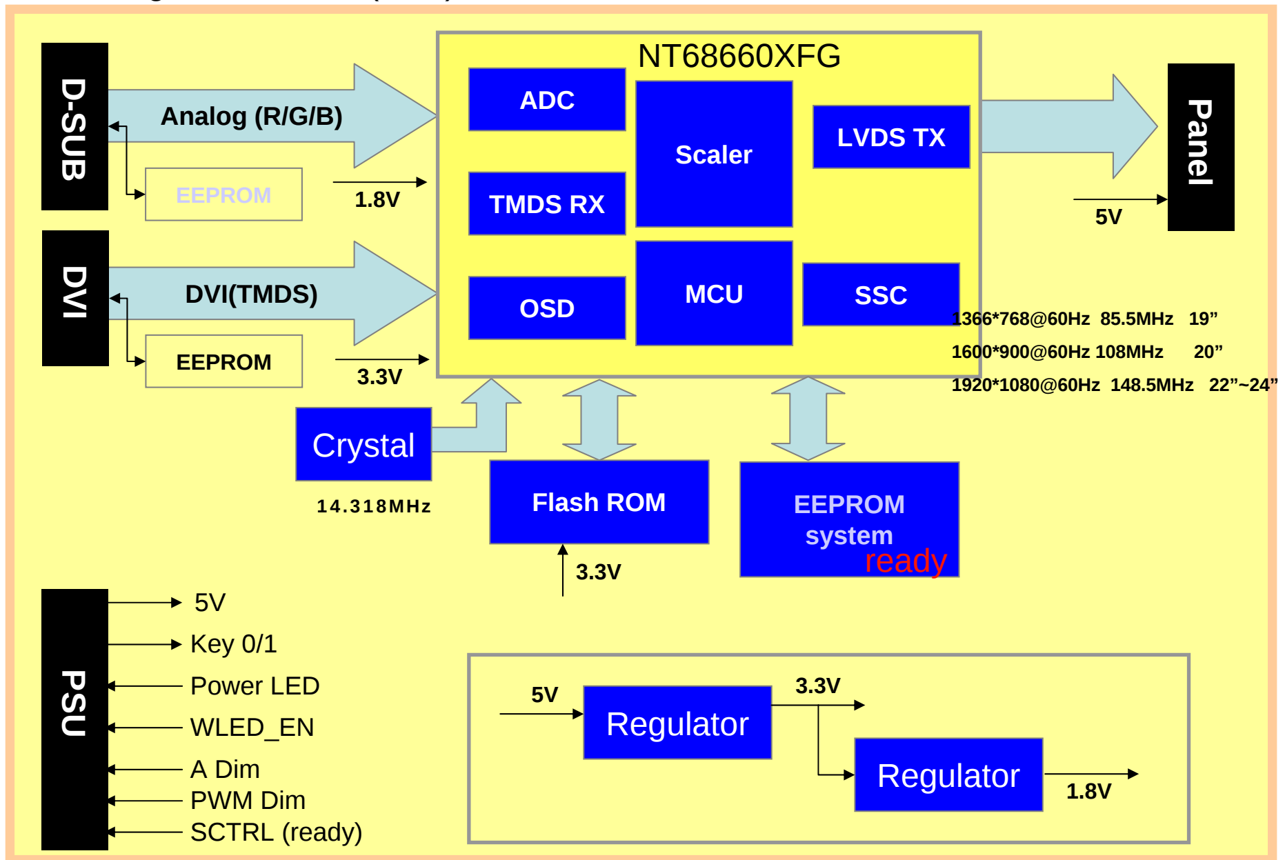
Block diagram for E41T (NVT)
