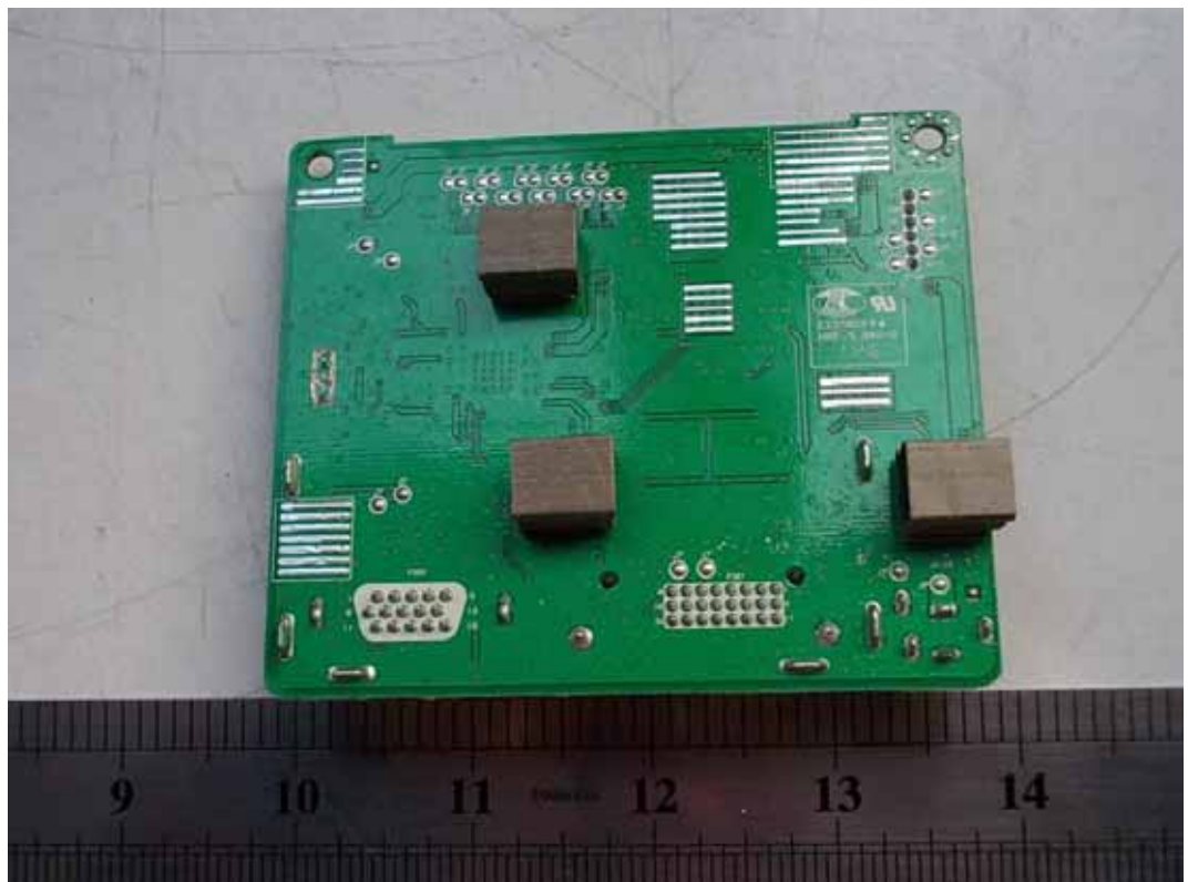
FIGURE 4 LCD MONITOR (M/N: E2242TA) MAIN BOARD (SOLDERED SIDE)
