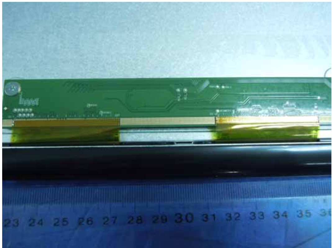
FIGURE 12 LCD MONITOR (M/N: E2242VA) LCD PANEL BOARD-1 (SOLDERED SIDE)
