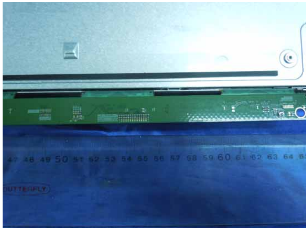
FIGURE 11 LCD MONITOR (M/N: E2242VA) LCD PANEL BOARD-3 (COMPONENT SIDE)
