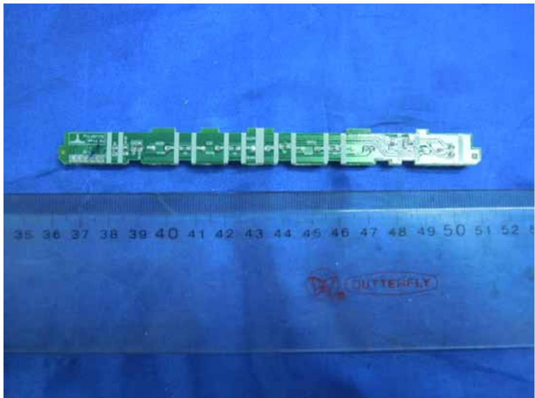
FIGURE 8 LCD MONITOR (M/N: E2242VA) KEY BOARD (SOLDERED SIDE)
