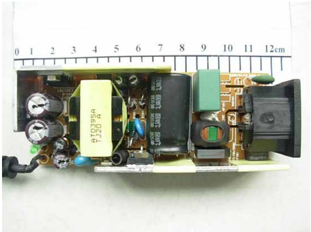
FIGURE 11 LCD MONITOR (M/N: E2250SV) ADAPTER (MAIN BOARD – COMPONENT SIDE)
