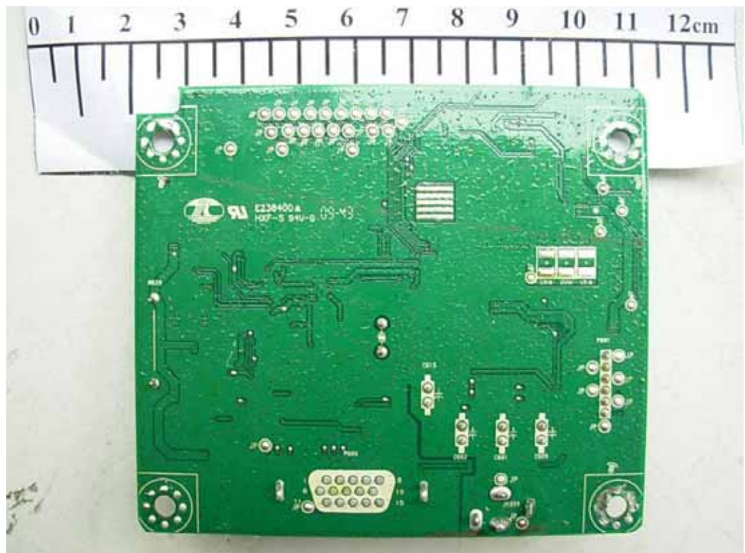
FIGURE 3 LCD MONITOR (M/N: E2250SV) MAIN BOARD (SOLDERED SIDE)
