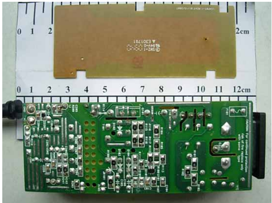
FIGURE 15 LCD MONITOR (M/N: E2250TV) ADAPTER #1 (MAIN BOARD –SOLDERED SIDE)
