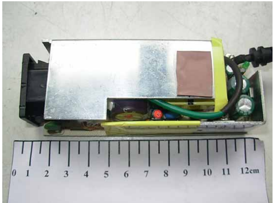
FIGURE 20 LCD MONITOR (M/N: E2250TV) ADAPTER #2 (MAIN BOARD – COMPONENT SIDE)
