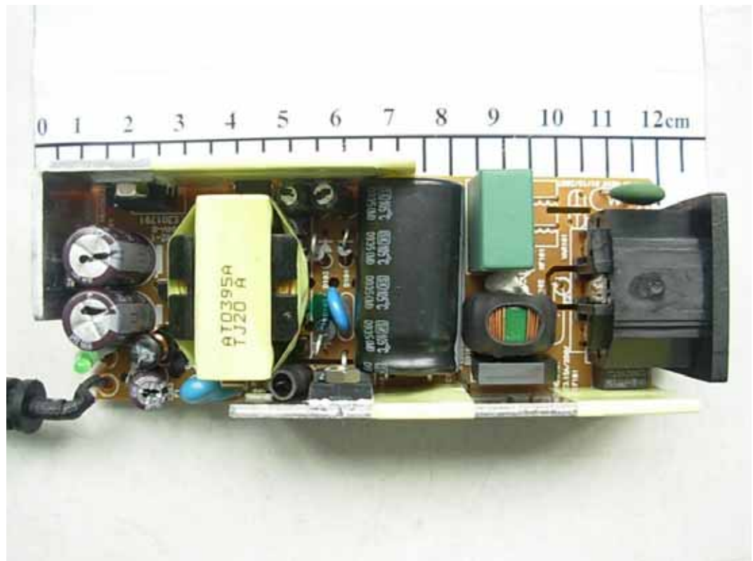
FIGURE 13 LCD MONITOR (M/N: E2250VV) ADAPTER (MAIN BOARD – COMPONENT SIDE)
