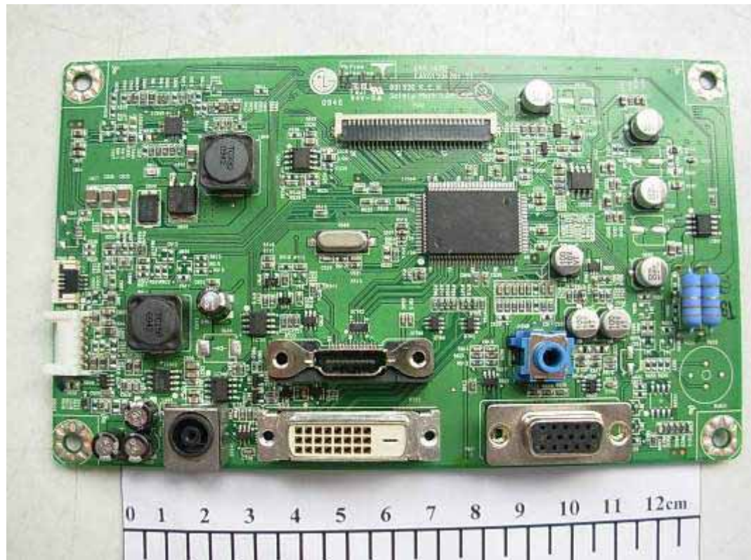
FIGURE 4 LCD MONITOR (M/N: E2250VV) MAIN BOARD (COMPONENT SIDE)
