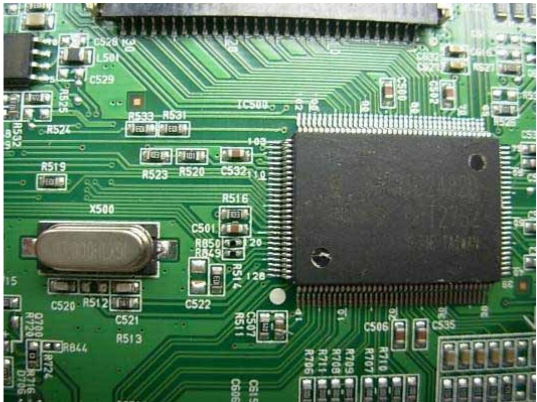
FIGURE 6 LCD MONITOR (M/N: E2250VV) CHIP & CRYSTAL ON MAIN BOARD
