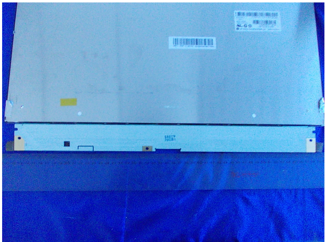
FIGURE 9 LCD MONITOR (M/N: E2251SZ) LCD PANEL CONTROL BOARD (SOLDERED SIDE)
