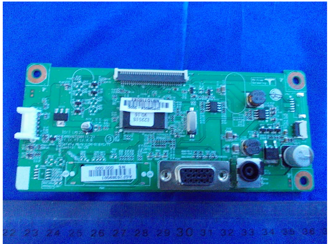
FIGURE 3 LCD MONITOR (M/N: E2251SZ) MAIN BOARD (COMPONENT SIDE)
