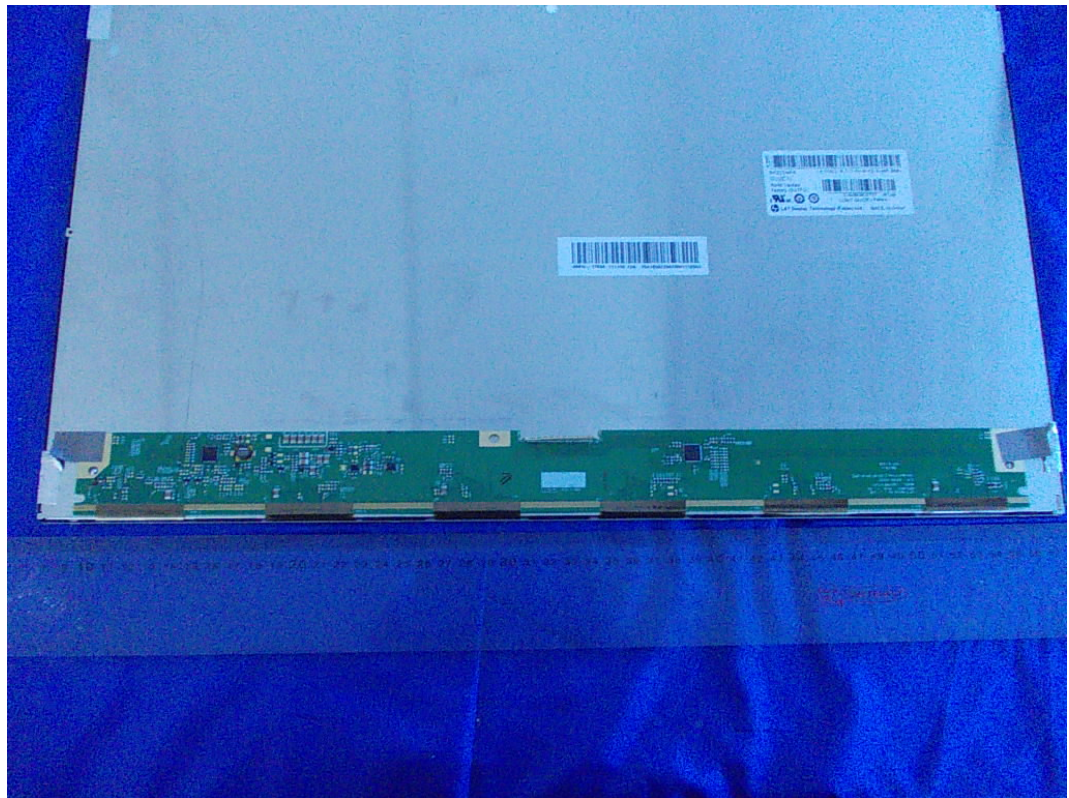
FIGURE 8 LCD MONITOR (M/N: E2251SZ) LCD PANEL CONTROL BOARD (COMPONENT SIDE)
