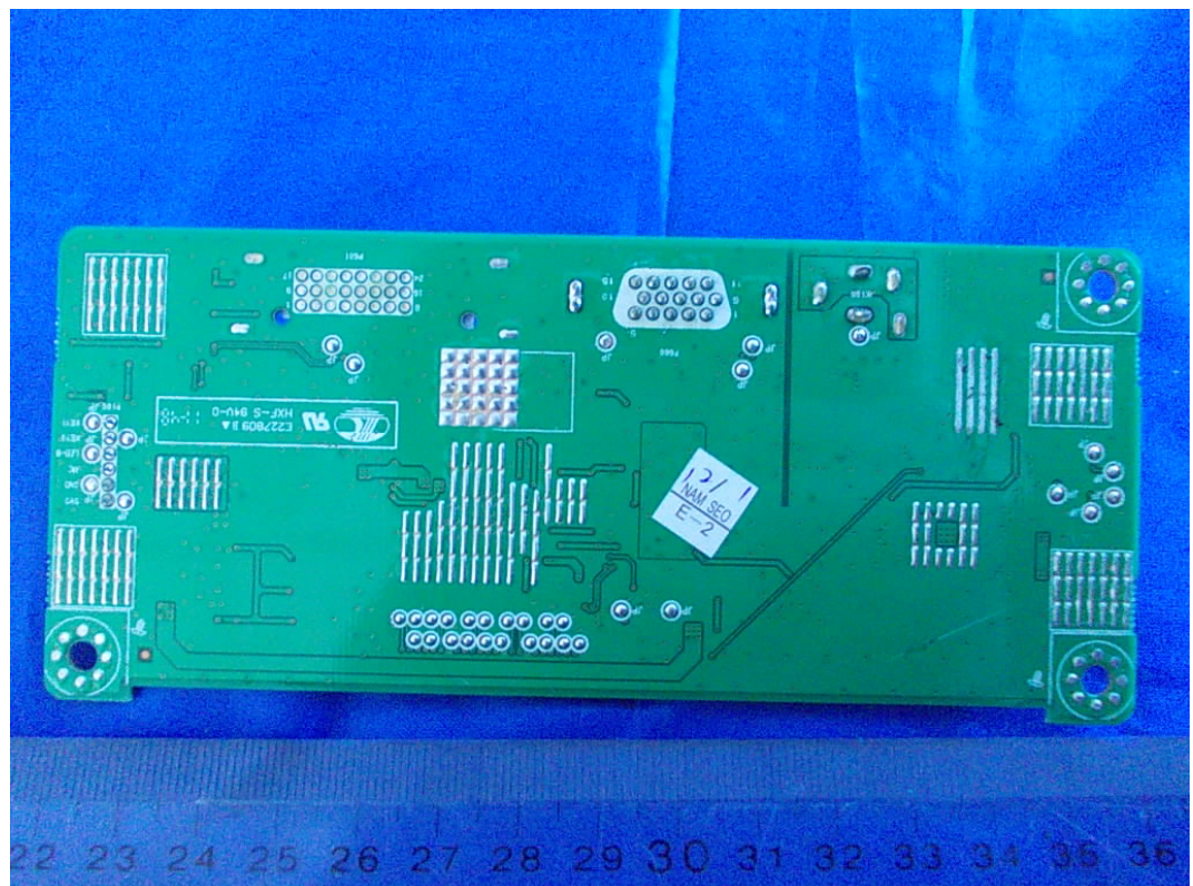
FIGURE 4 LCD MONITOR (M/N: E2251SZ) MAIN BOARD (COMPONENT SIDE)
