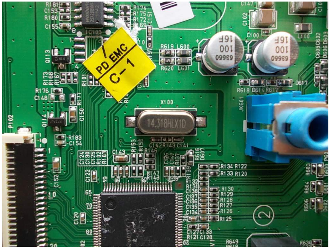
FIGURE 4 LCD MONITOR (M/N: E2251VZ) CRYSTAL ON MAIN BOARD
