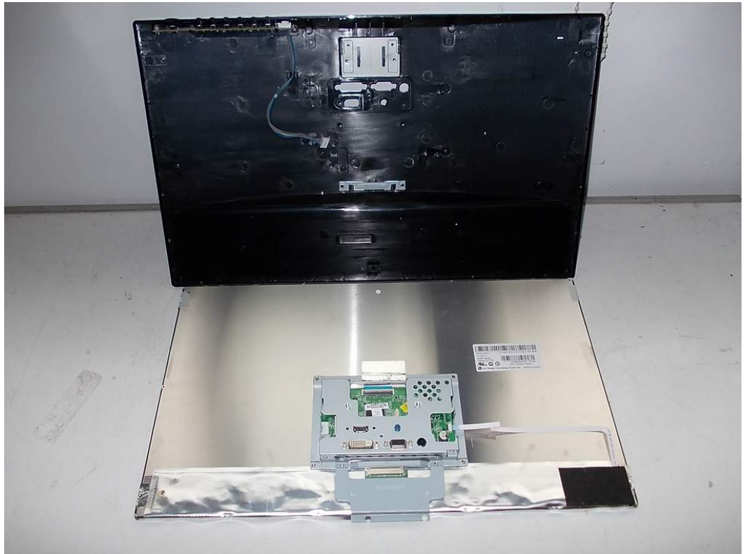
FIGURE 1 LCD MONITOR (M/N: E2251VZ) COVER REMOVED
