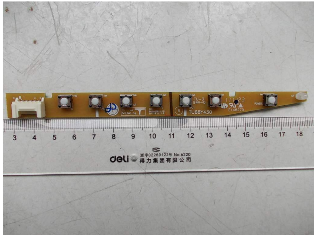
FIGURE 6 LCD MONITOR (M/N: E2251VZ) KEY BOARD (COMPONENT SIDE)
