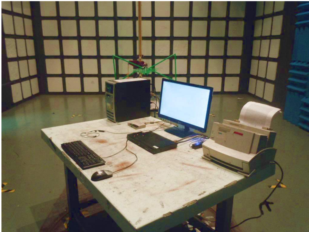
SETUP WITH MAXIMUM DETECTED EMISSION AT HORIZONTAL POLARIZATION (TEST MODE: DVI 640*480@60Hz Adapter #1)
