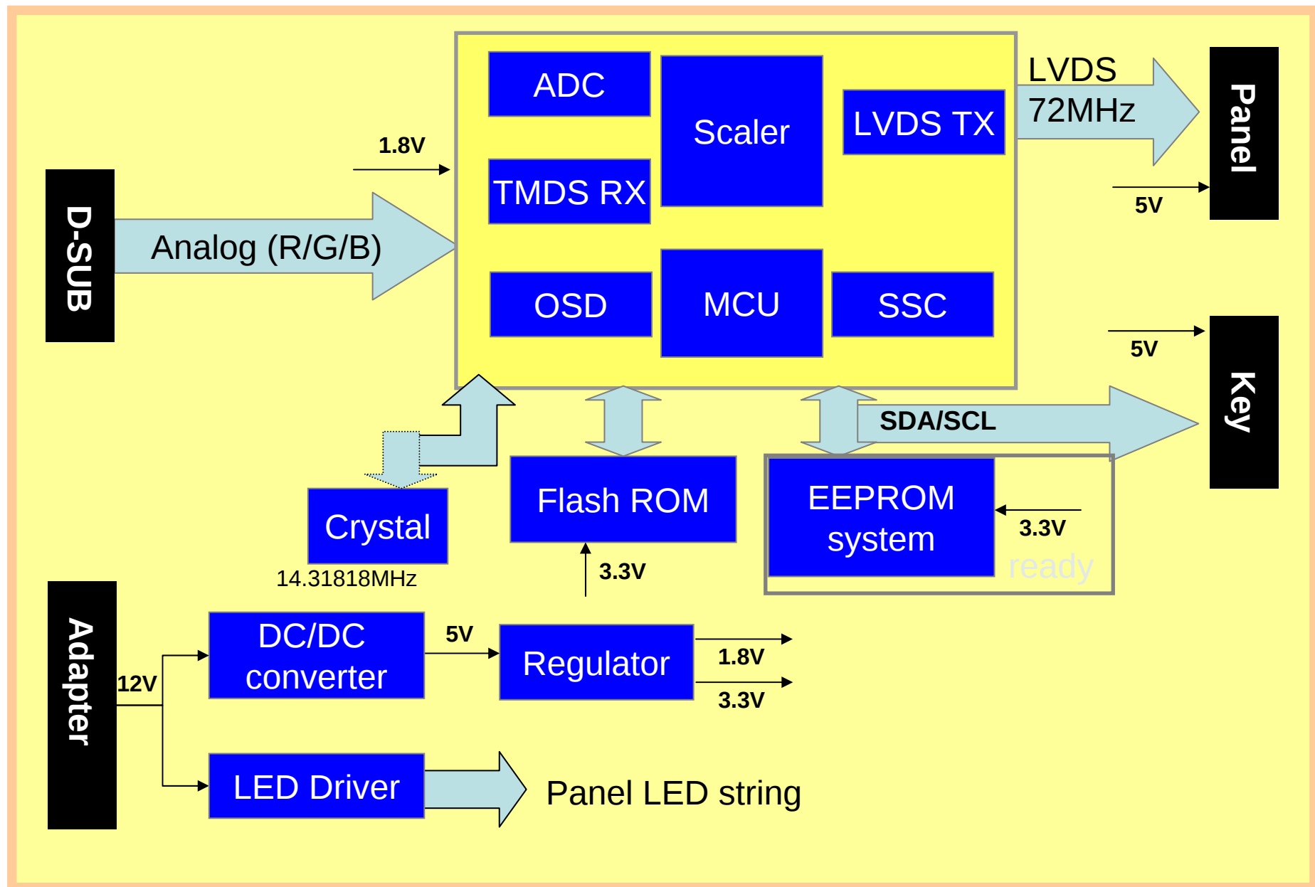
Block diagram for E40S
