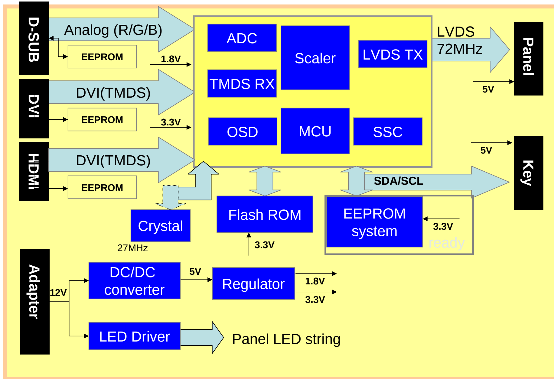
Block diagram for E40V
