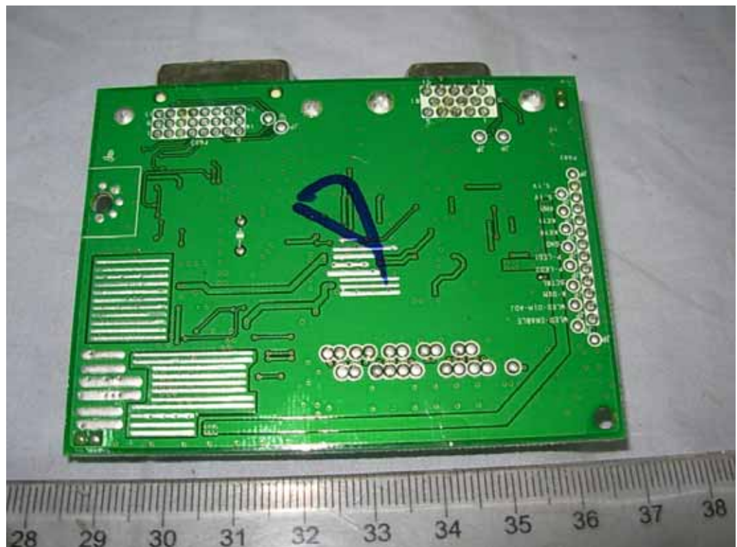
FIGURE 6 LCD MONITOR (M/N: E2341TX) MAIN BOARD (SOLDERED SIDE)
