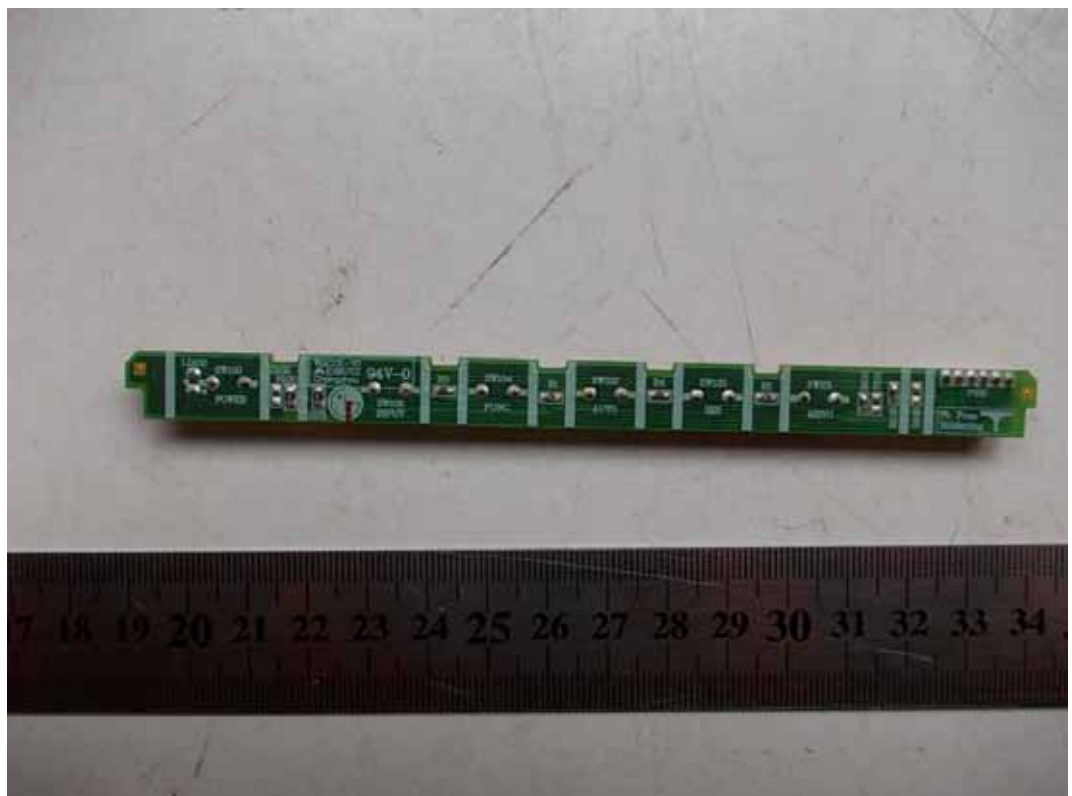
FIGURE 7 LCD MONITOR (M/N: E2342VA) KEY BOARD (SOLDERED SIDE)
