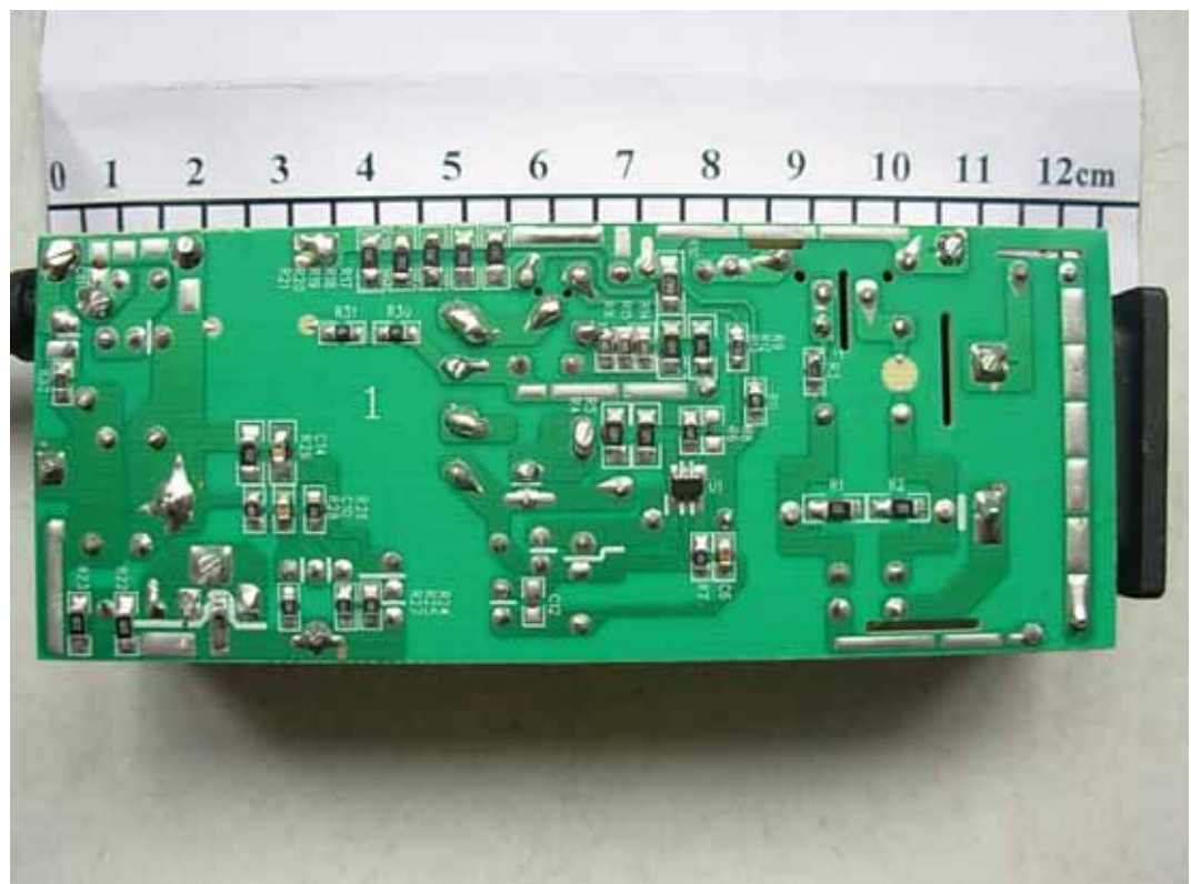
FIGURE 12 LCD MONITOR (M/N: E2350SV) ADAPTER (MAIN BOARD –SOLDERED SIDE)
