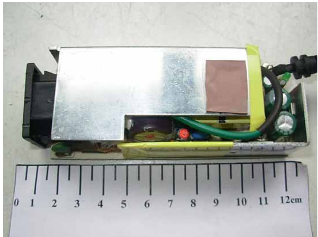
FIGURE 11 LCD MONITOR (M/N: E2350SV) ADAPTER (MAIN BOARD – COMPONENT SIDE)
