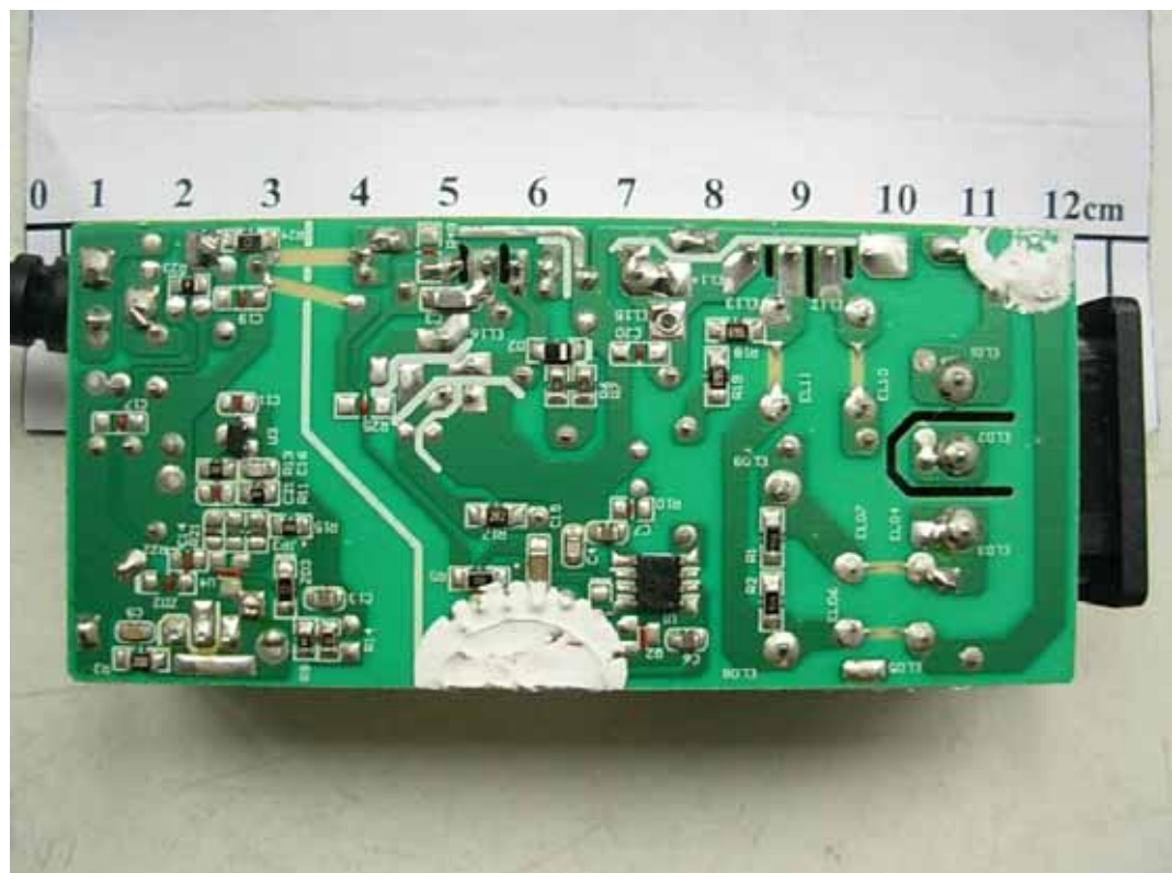
FIGURE 21 LCD MONITOR (M/N: E2350VV) ADAPTER #2 (MAIN BOARD – SOLDERED SIDE)
