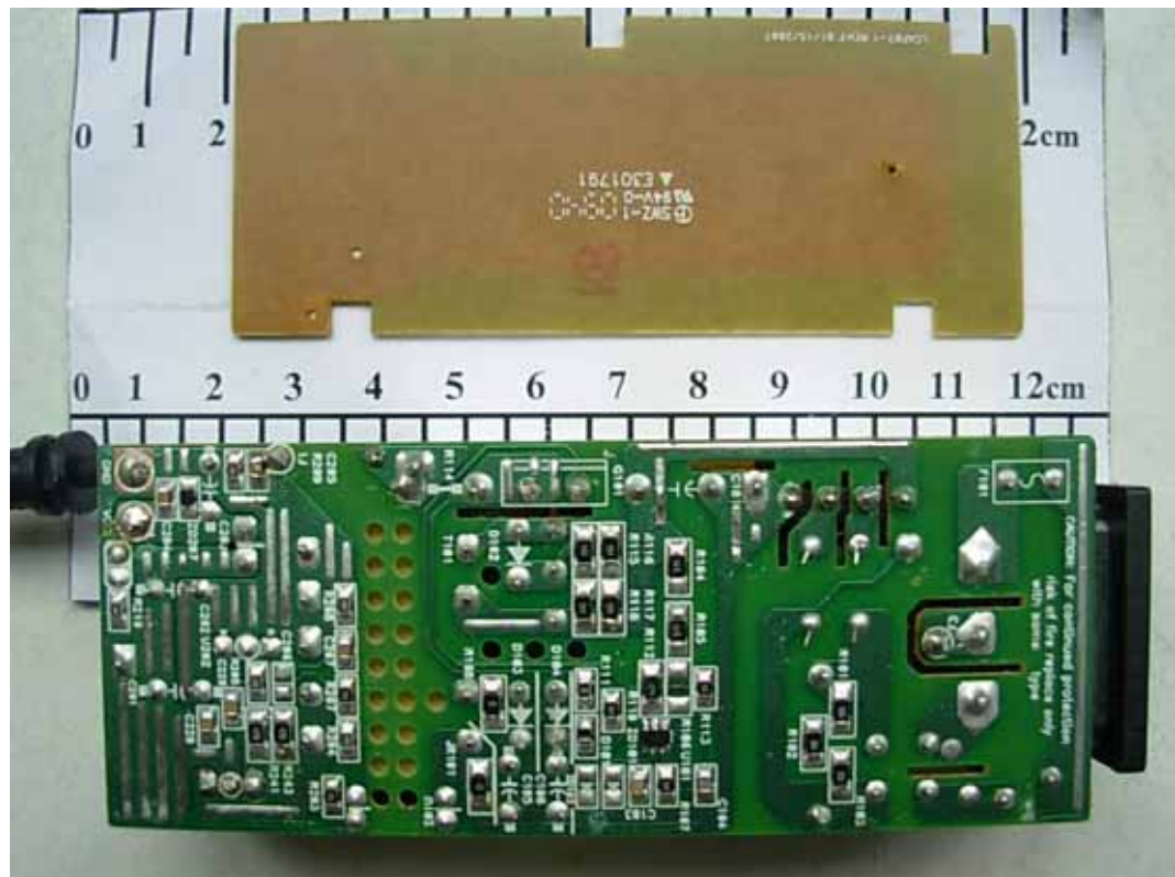
FIGURE 15 LCD MONITOR (M/N: E2350VV) ADAPTER #1 (MAIN BOARD –SOLDERED SIDE)
