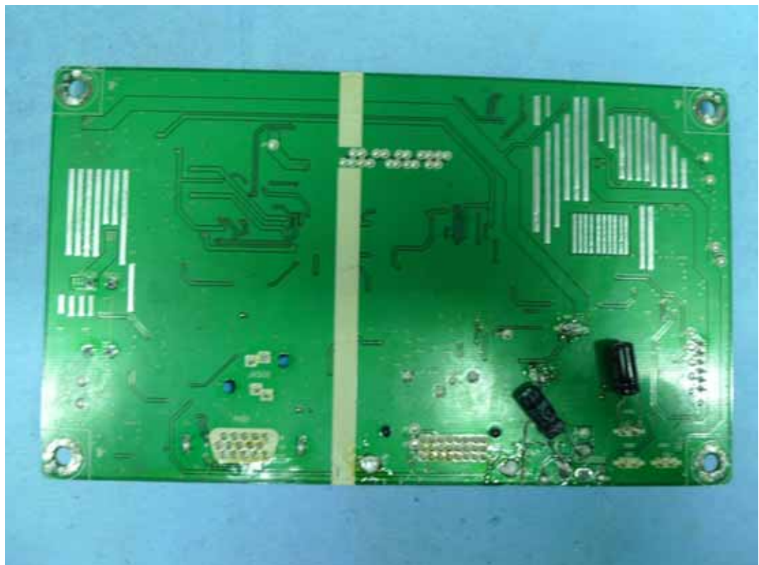
FIGURE 7 LCD MONITOR (M/N: E2350TV) MAIN BOARD (SOLDERED SIDE)
