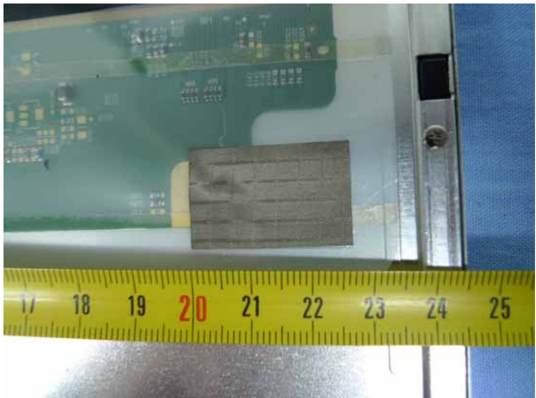
FIGURE 13 LCD MONITOR (M/N: E2350VV) DEBUG #4
