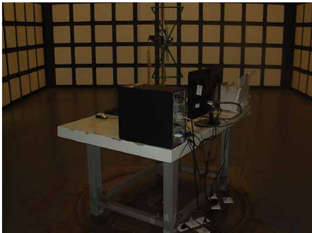
SETUP WITH MAXIMUM DETECTED EMISSION AT VERTICAL POLARIZATION (TEST MODE: D-SUB1680*1050@60Hz) (ADAPTER: LCAP07F)
