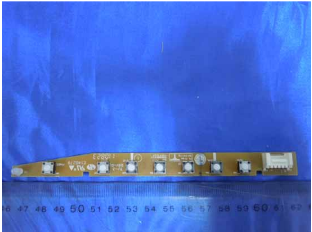
FIGURE 6 LCD MONITOR (M/N: E2351VZ) KEY BOARD (COMPONENT SIDE)
