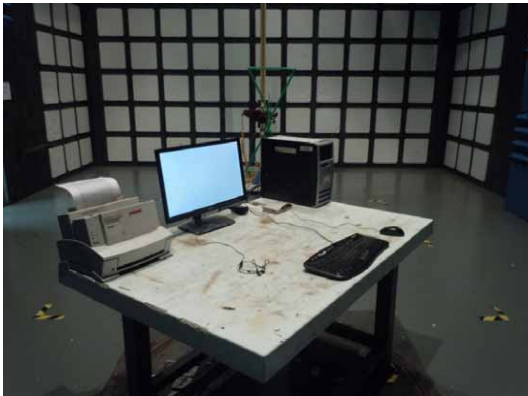
SETUP WITH MAXIMUM DETECTED EMISSION AT VERTICAL POLARIZATION (TEST MODE: D-SUB 1920*1080@60Hz Adapter #1)
