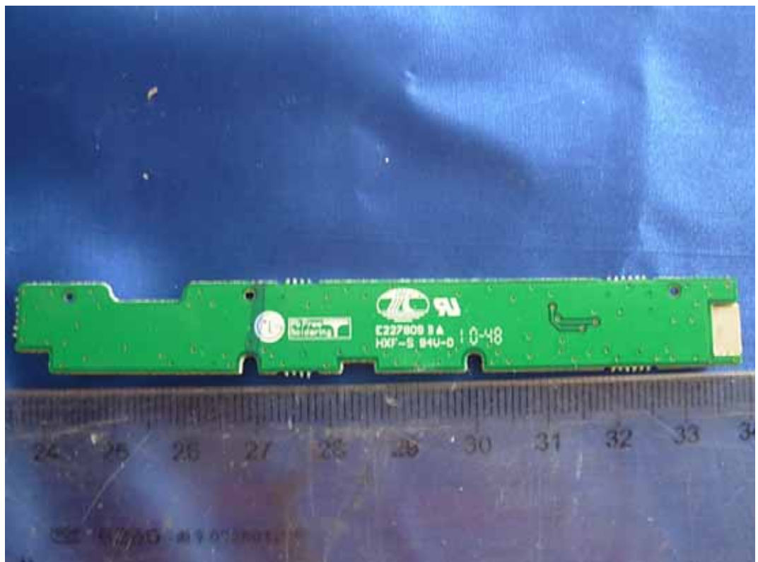
FIGURE 11 LCD MONITOR (M/N: E2411PUX) KEY BOARD (SOLDERED SIDE)
