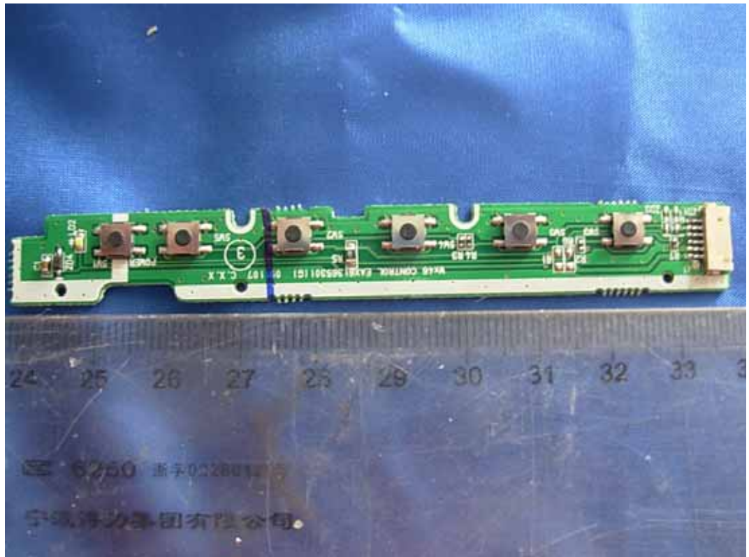
FIGURE 10 LCD MONITOR (M/N: E2411PUX) KEY BOARD (COMPONENT SIDE)
