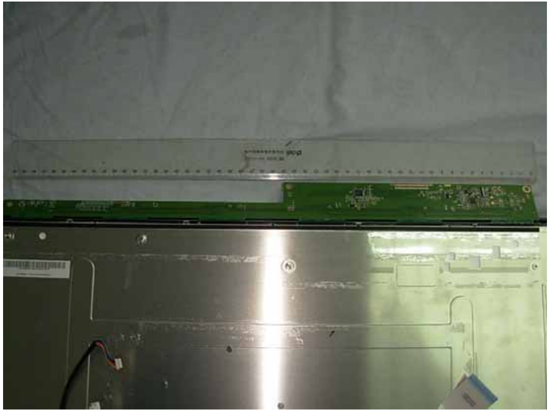
FIGURE 8 LCD MONITOR (M/N: E2441VX) DISPLAY BOARD (COMPONENT SIDE)
