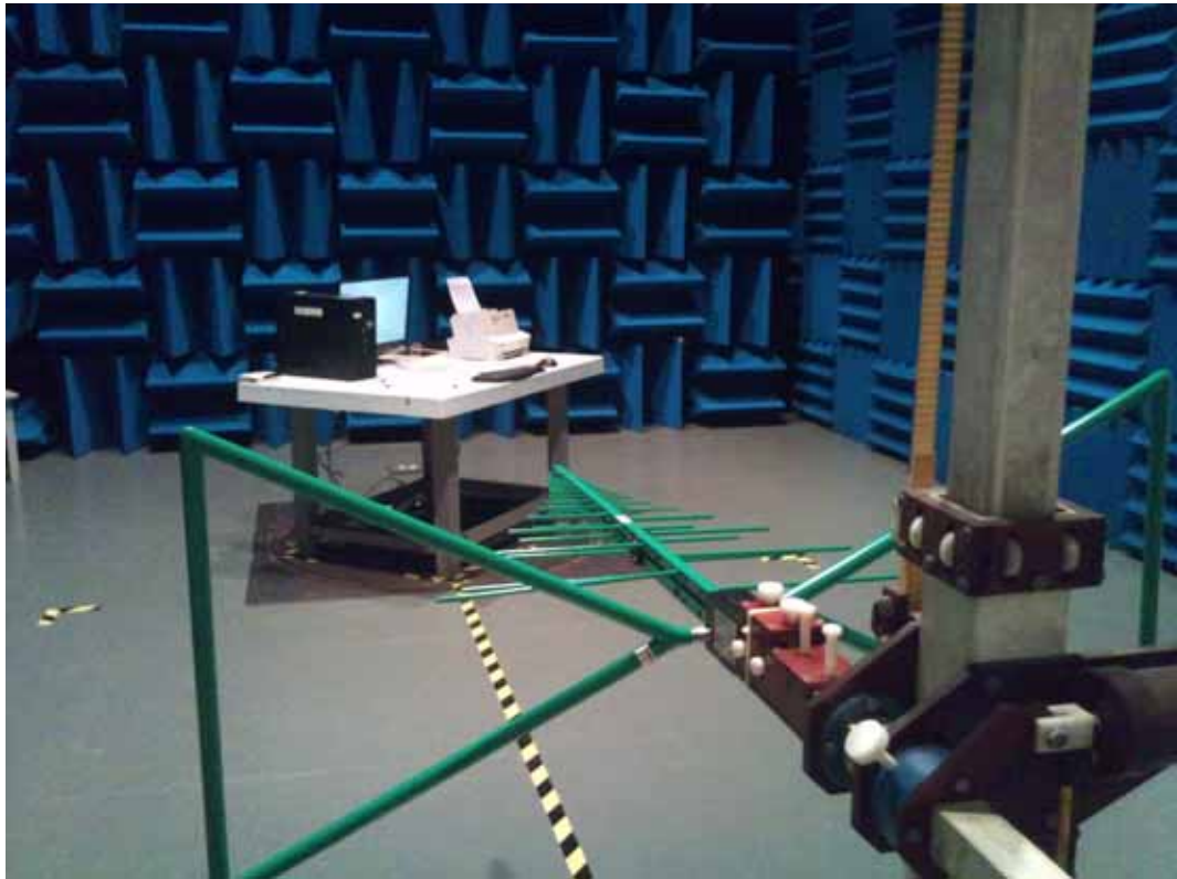
SETUP WITH MAXIMUM DETECTED EMISSION AT HORIZONTAL POLARIZATION (TEST MODE: DVI 1280*1024@75Hz)
