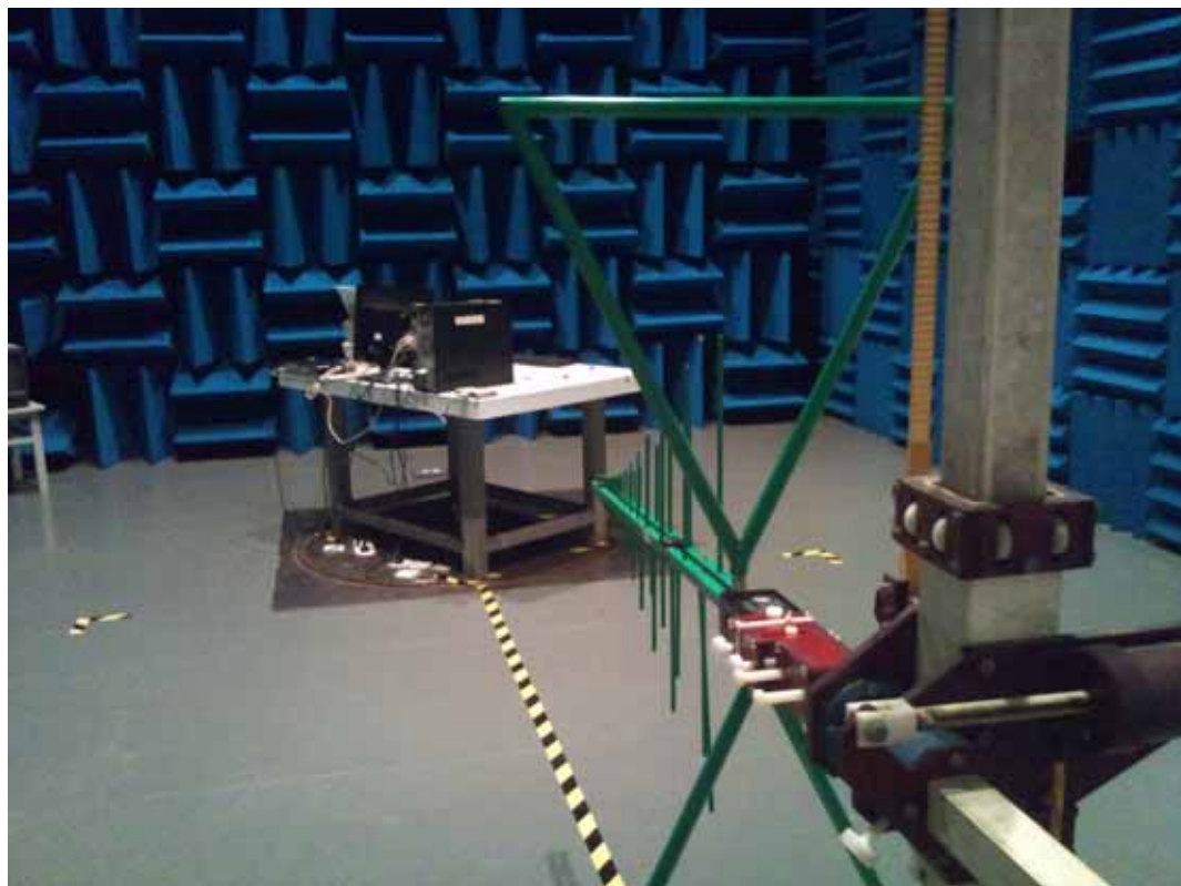
SETUP WITH MAXIMUM DETECTED EMISSION AT VERTICAL POLARIZATION (TEST MODE: DVI 1280*1024@75Hz)
