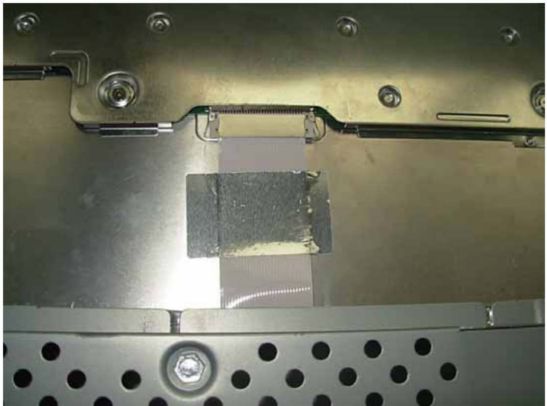
FIGURE 13 LCD MONITOR (M/N: E2541TX) DEBUG #2
