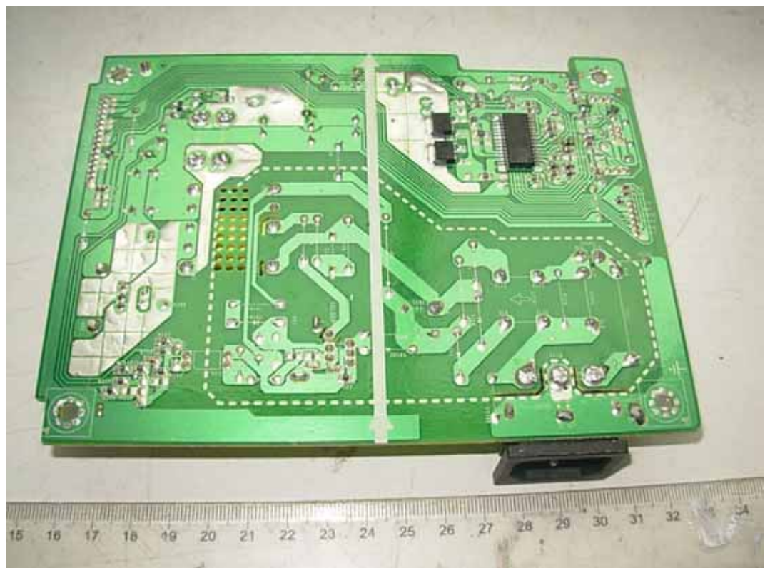
FIGURE 7 LCD MONITOR (M/N: E2541TX) POWER BOARD (SOLDERED SIDE)
