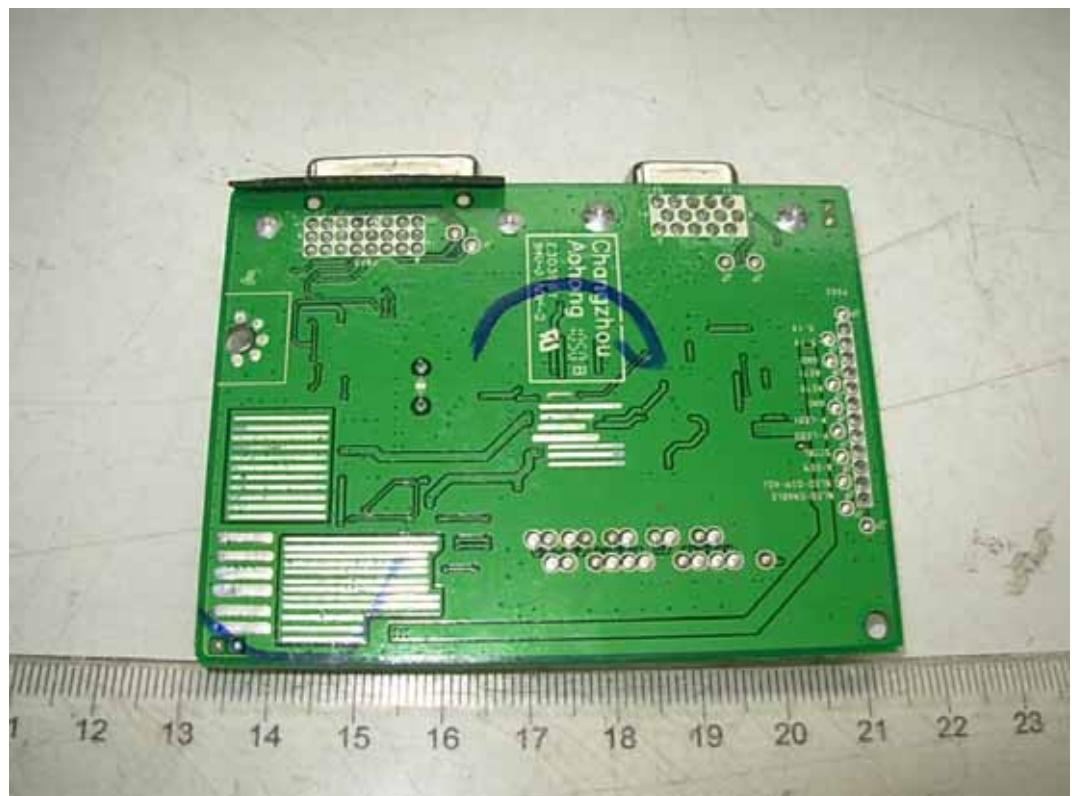
FIGURE 4 LCD MONITOR (M/N: E2541TX) MAIN BOARD (COMPONENT SIDE)
